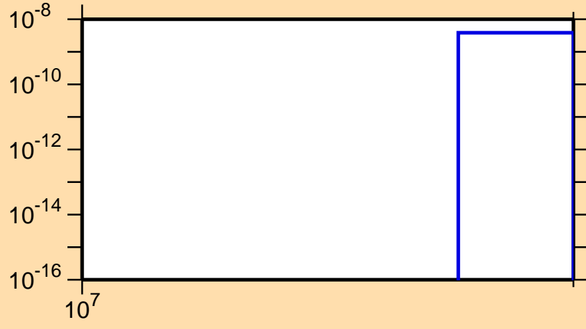
\sigma vs. E for ^{206}\text{Rn}(n,3n\alpha)
