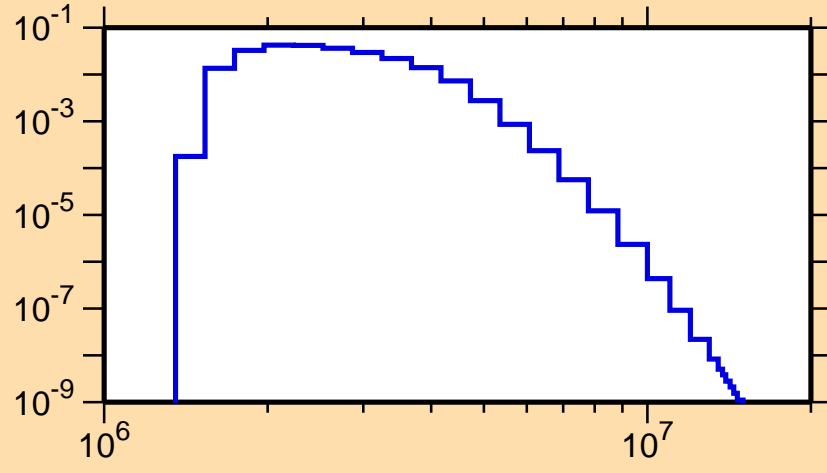
\sigma vs. E for ^{206}\text{Rn}(n,n_3)
