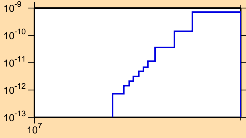
\sigma vs. E for ^{206}\text{Rn}(\text{mt117})
