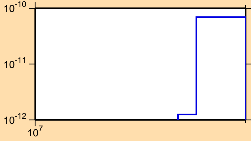
\sigma vs. E for ^{206}\text{Rn}(n,\text{pt})
