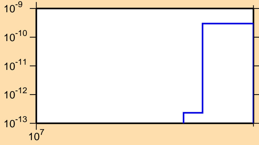
\sigma vs. E for ^{206}\text{Rn}(n,nt)
