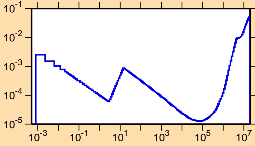
\sigma vs. E for ^{206}\text{Rn}(n,p)
