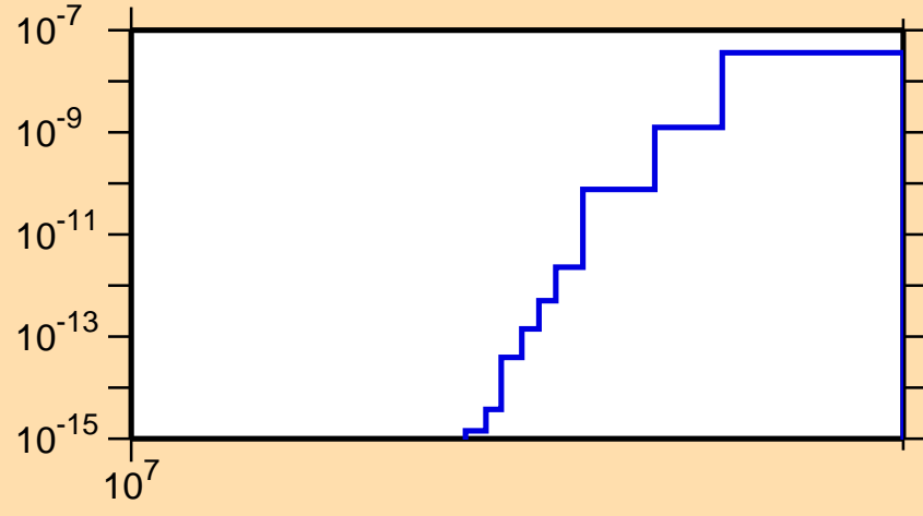
\sigma vs. E for ^{206}\text{Rn}(n,nd)
