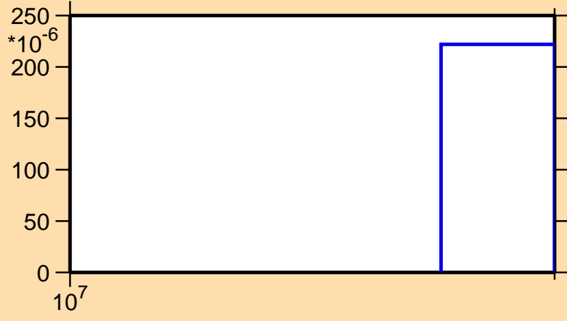
\sigma vs. E for ^{206}\text{Rn}(n,3n)
