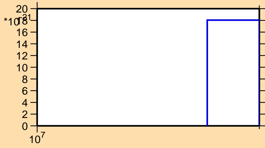
\sigma vs. E for ^{206}\text{Rn} (mt 11)
