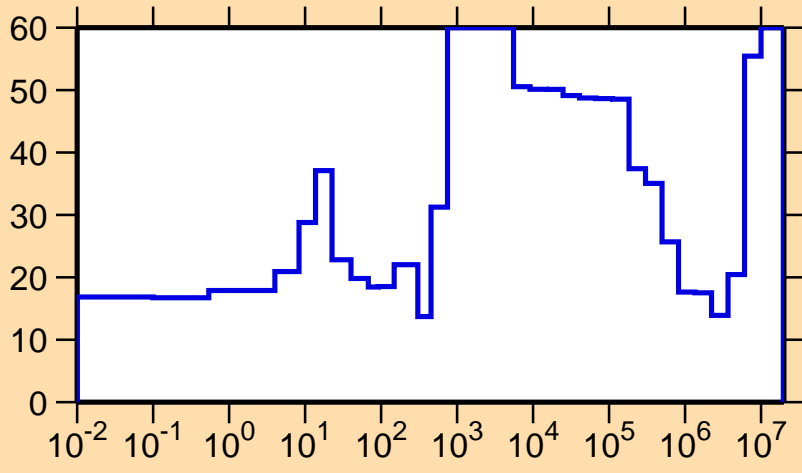
\Delta\sigma/\sigma vs. E for ^{206}\text{Rn}(n,\gamma)
