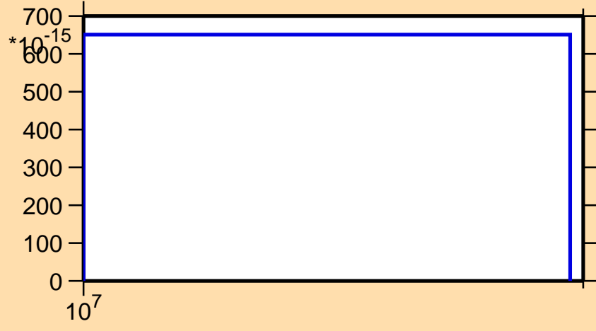
\sigma vs. E for ^{206}\text{Rn}(n,\text{pt})
