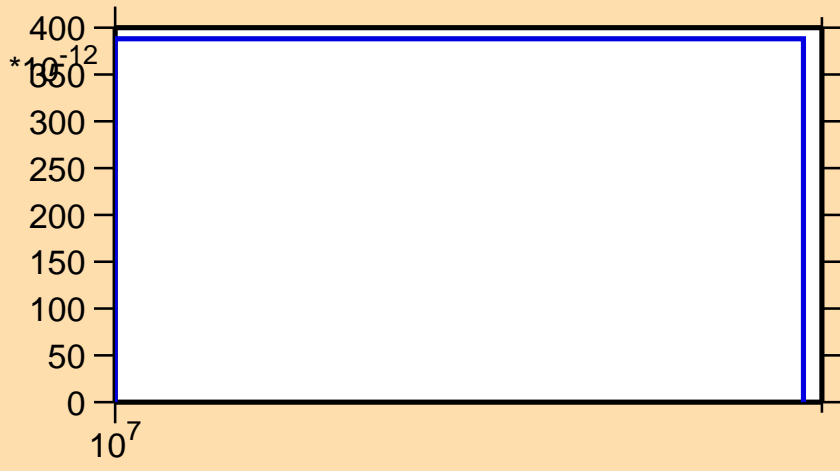
\sigma vs. E for ^{206}\text{Rn}(n,\text{nd})
