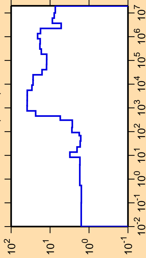
\Delta\sigma/\sigma vs. E for ^{206}\text{Rn}(n,\text{el.})
