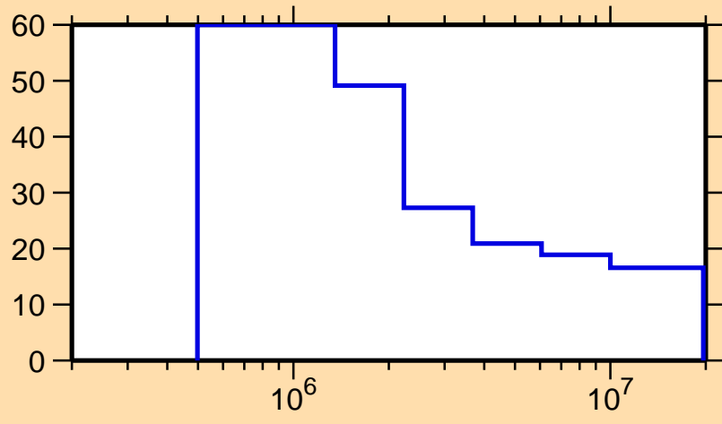
\Delta\sigma/\sigma vs. E for ^{206}\text{Rn}(n,n_1)
