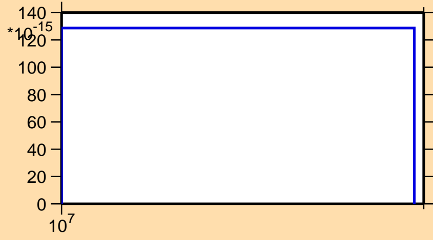
\sigma vs. E for ^{206}\text{Rn} (mt 34)
