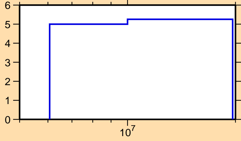
\Delta\sigma/\sigma vs. E for ^{206}\text{Rn}(n,\text{nonel.})
