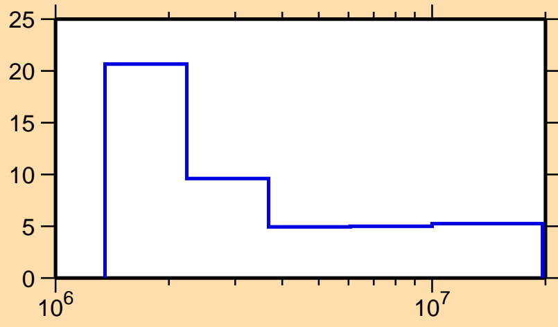
\Delta\sigma/\sigma vs. E for ^{206}\text{Rn}(n,\text{nonel.})
