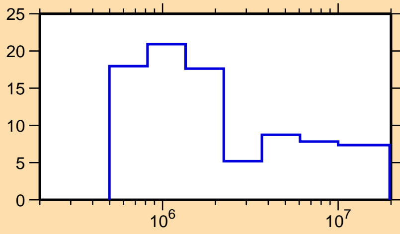
\Delta\sigma/\sigma vs. E for ^{206}\text{Rn}(n,\text{el.})
