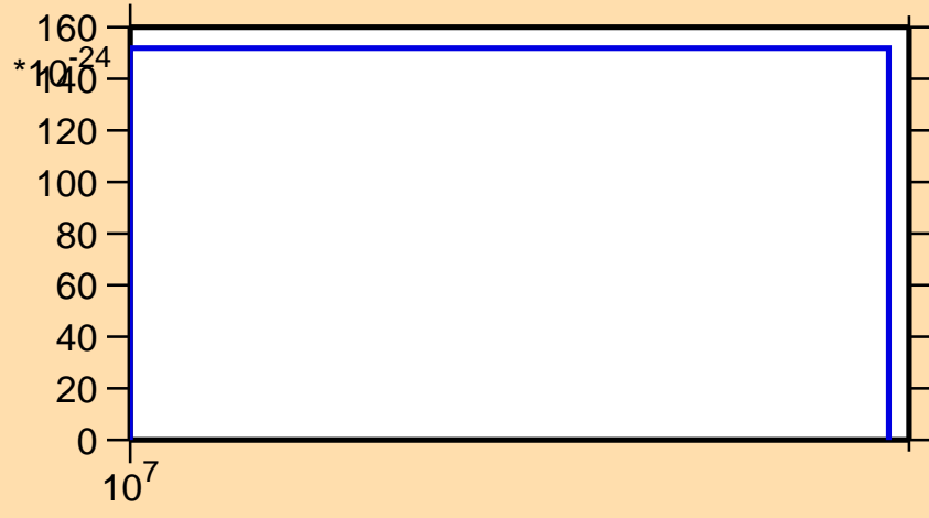
\sigma vs. E for ^{206}\text{Rn} (mt 11)
