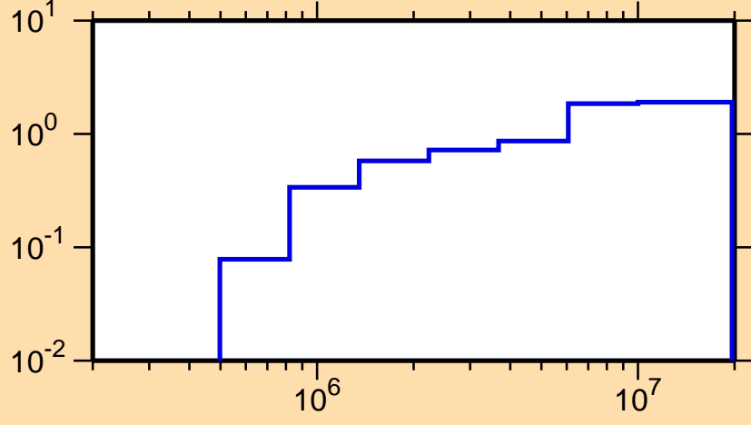
\sigma vs. E for ^{206}\text{Rn}(n,\text{inel.})
