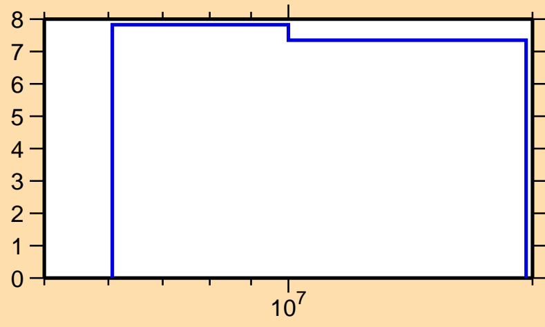
\Delta\sigma/\sigma vs. E for ^{206}\text{Rn}(n,\text{el.})
