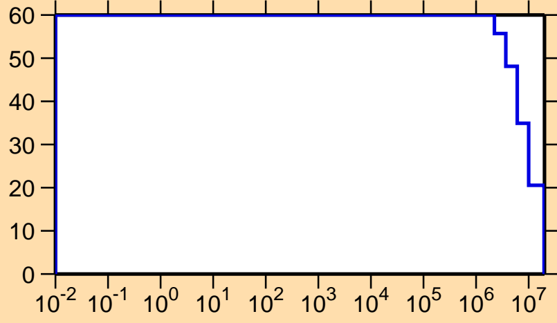
\Delta\sigma/\sigma vs. E for ^{206}\text{Rn}(n,p)
