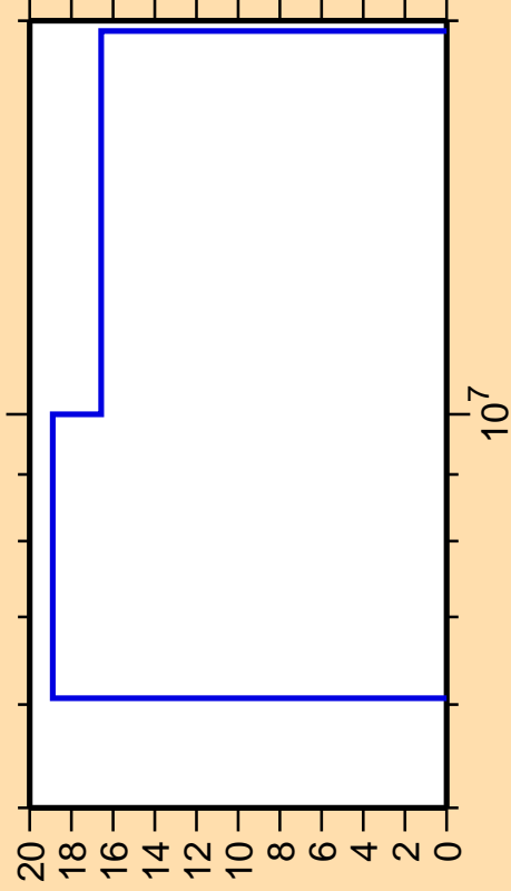
\Delta\sigma/\sigma vs. E for ^{206}\text{Rn}(n,n_1)
