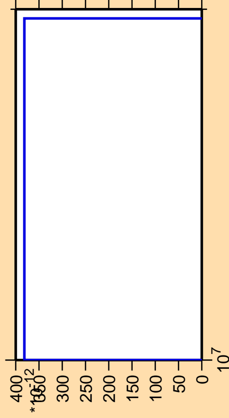
\Delta\sigma/\sigma vs. E for ^{206}\text{Rn} (mt 11)
