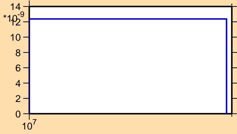
\sigma vs. E for ^{206}\text{Rn}(n,2np)
