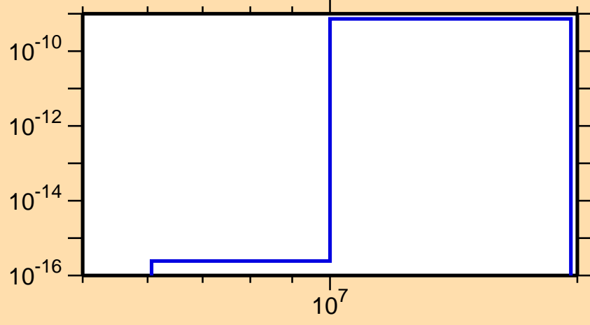
\sigma vs. E for ^{206}\text{Rn} (mt 45)
