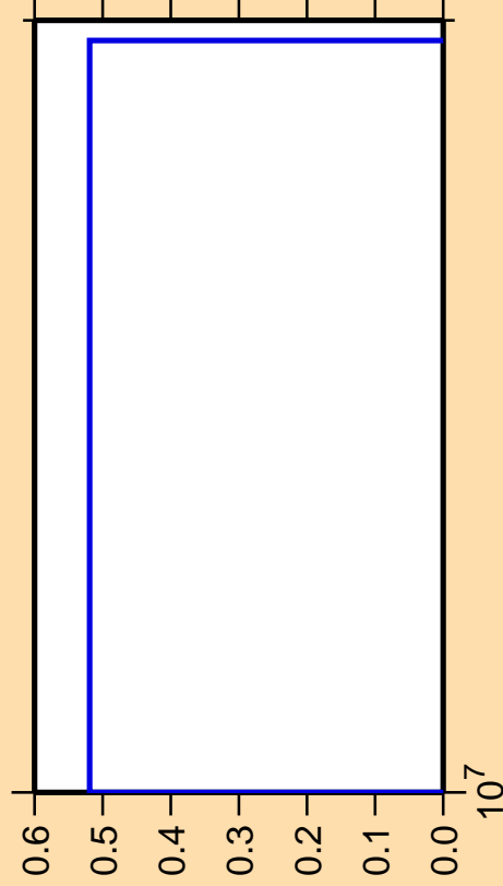
\Delta\sigma/\sigma vs. E for ^{206}\text{Rn} (mt 34)
