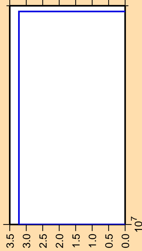
\Delta\sigma/\sigma vs. E for ^{206}\text{Rn}(n,\text{pt})
