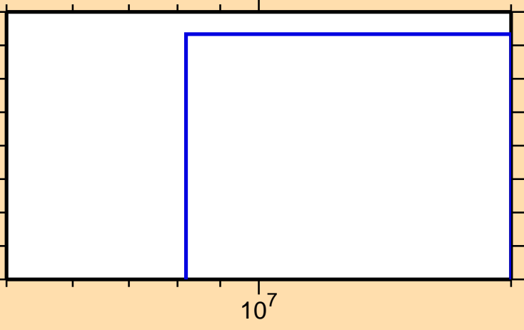
\sigma vs. E for ^{206}\text{Rn}(\text{mt 11})
