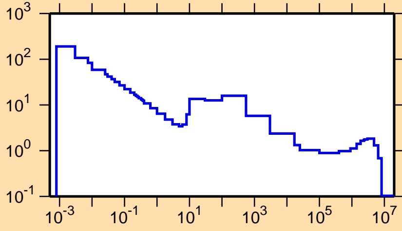
\sigma vs. E for ^{206}\text{Rn}(n,\gamma)
