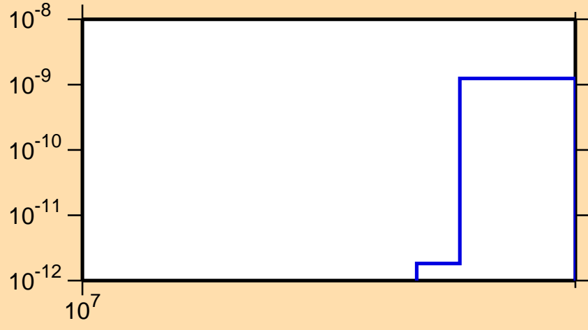
\sigma vs. E for ^{207}\text{Rn}(n,nt)
