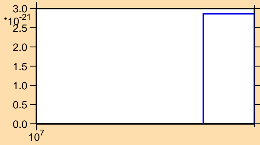
\sigma vs. E for ^{207}\text{Rn} (mt 11)
