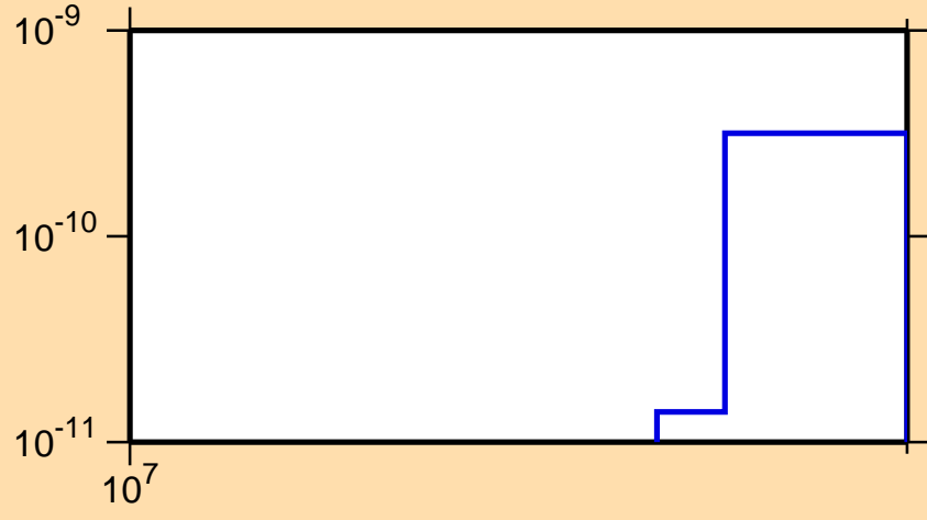
\sigma vs. E for ^{207}\text{Rn}(\text{mt 34})
