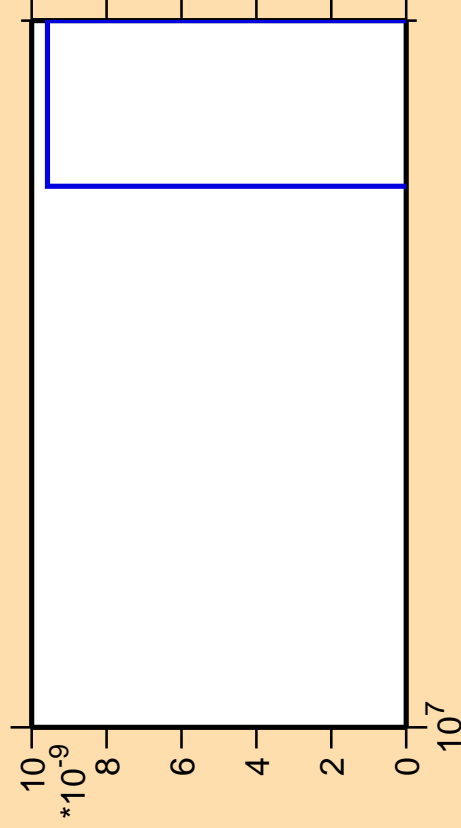
\Delta\sigma/\sigma vs. E for ^{207}\text{Rn} (mt 11)
