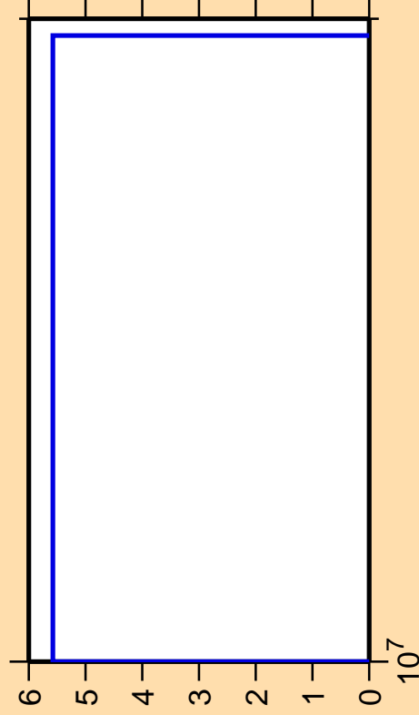
\Delta\sigma/\sigma vs. E for ^{207}\text{Rn} (mt 34)
