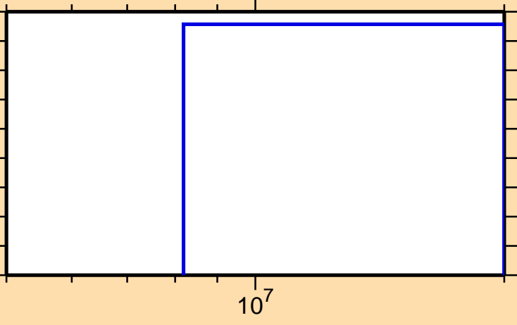
\sigma vs. E for ^{207}\text{Rn}(n,3n)
