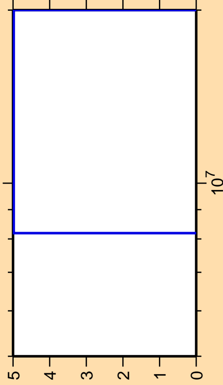
\Delta\sigma/\sigma vs. E for ^{207}\text{Rn}(\text{mt } 34)
