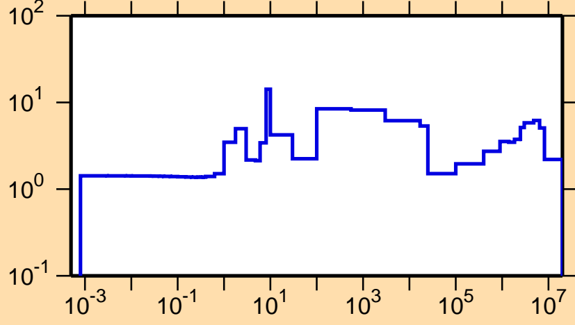
\Delta\sigma/\sigma vs. E for ^{207}\text{Rn}(n,\text{el.})
