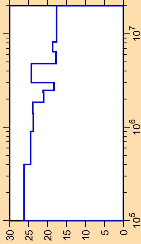
\Delta\sigma/\sigma vs. E for ^{207}\text{Rn}(n,n_3)
