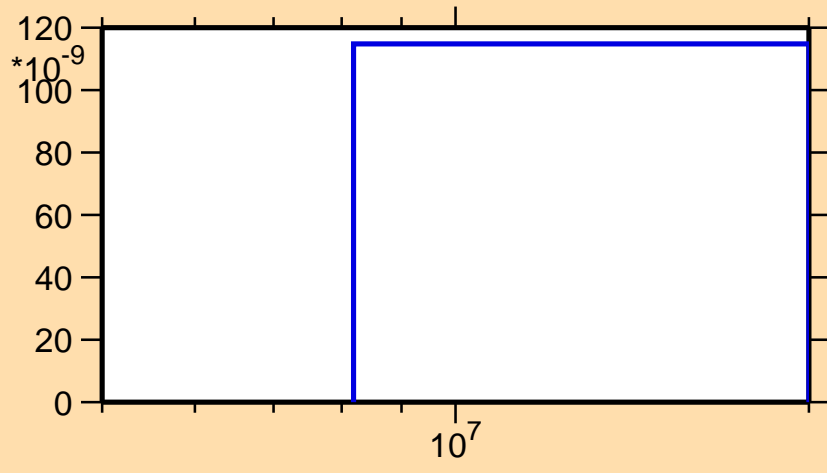
\sigma vs. E for ^{207}\text{Rn}(n,nd)
