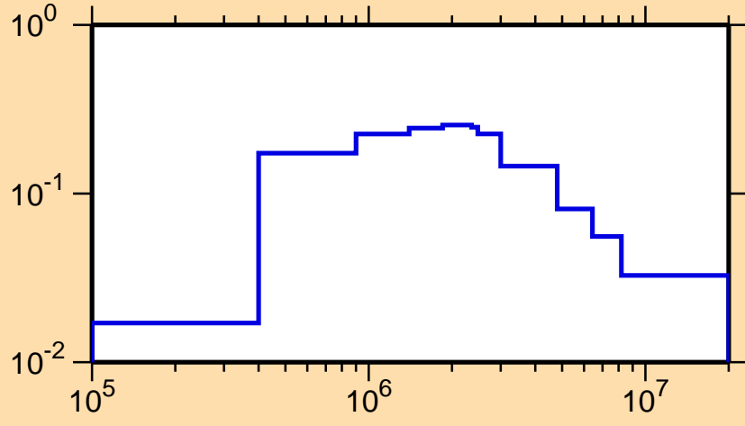
\sigma vs. E for ^{207}\text{Rn}(n,n_2)
