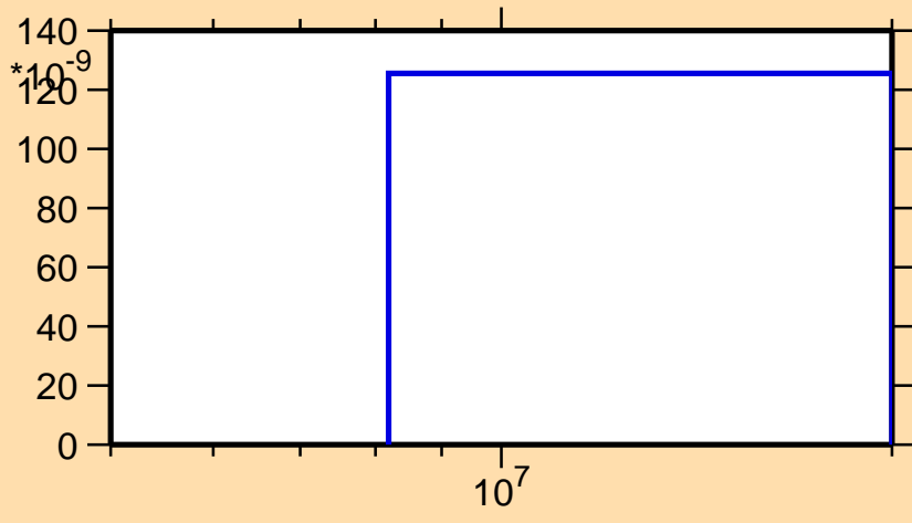
\sigma vs. E for ^{207}\text{Rn}(n,\text{He}3)
