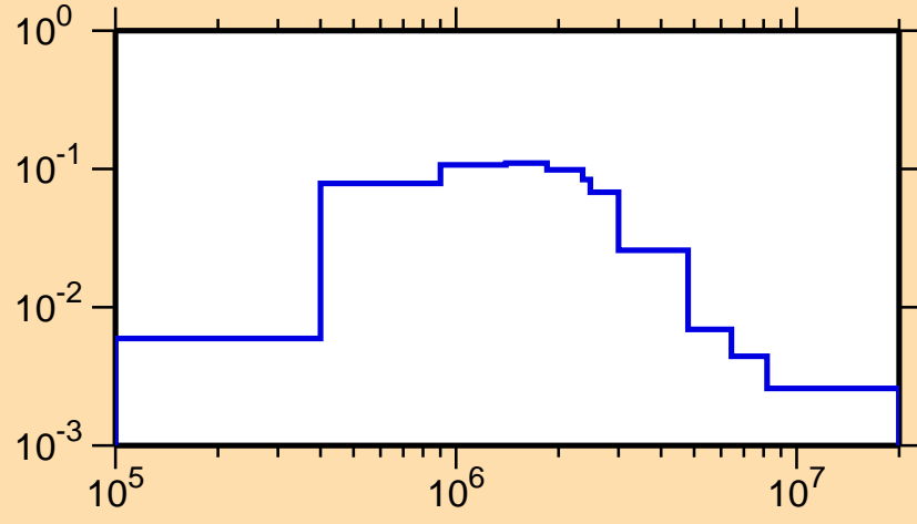
\sigma vs. E for ^{207}\text{Rn}(n,n_3)
