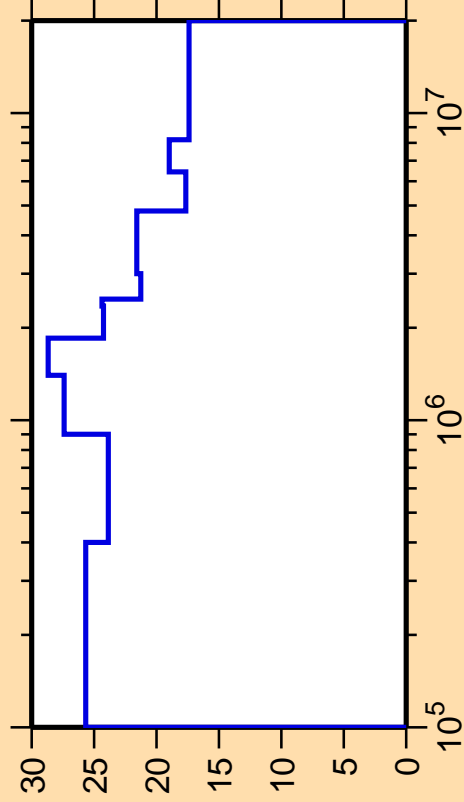
\Delta\sigma/\sigma vs. E for ^{207}\text{Rn}(n,n_2)
