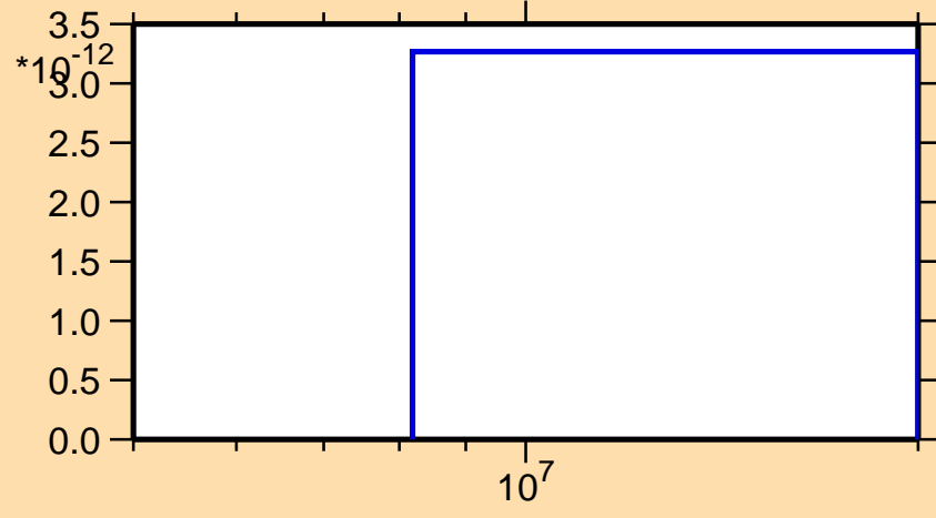
\sigma vs. E for ^{207}\text{Rn}(\text{mt } 34)
