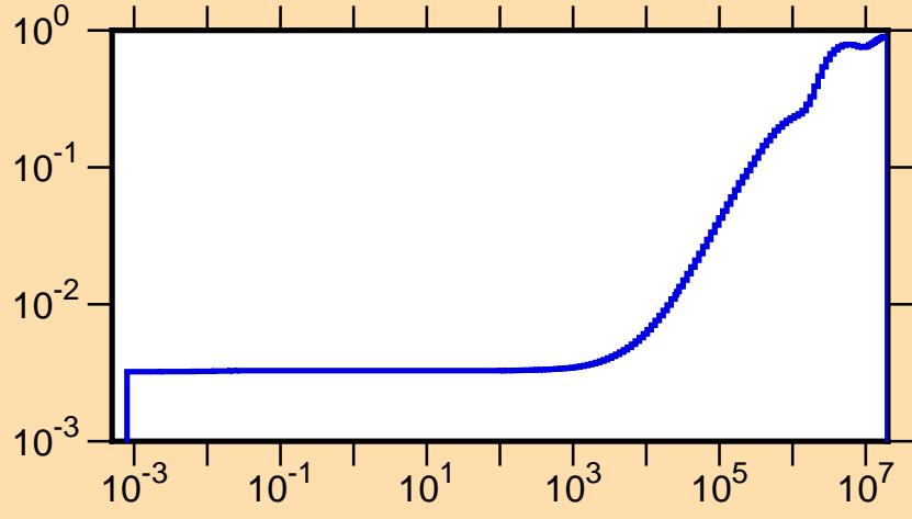
\mu vs. E for ^{209}\text{Rn}(\text{mt251})
