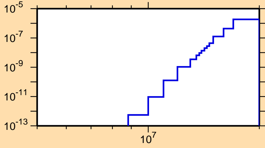
\sigma vs. E for ^{209}\text{Rn}(n,\text{He3})
