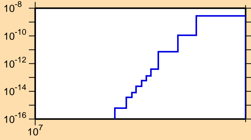
\sigma vs. E for ^{209}\text{Rn}(n,\text{pt})
