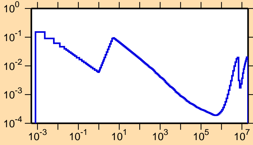
\sigma vs. E for ^{209}\text{Rn}(n,\alpha)
