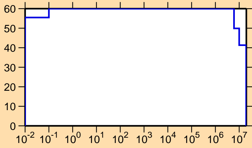
\Delta\sigma/\sigma vs. E for ^{209}\text{Rn}(n,p)
