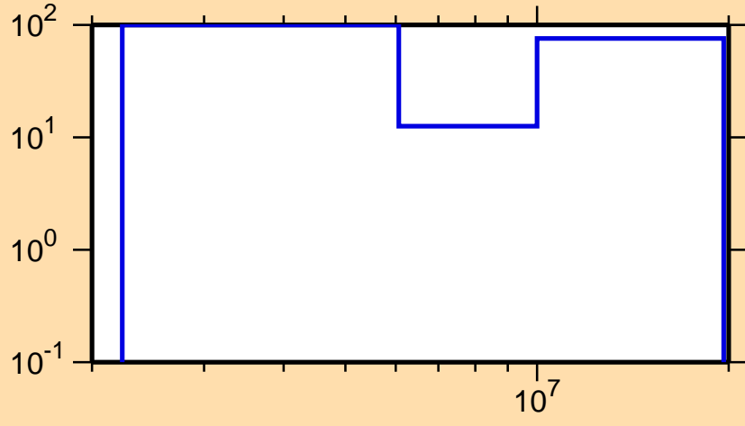
\Delta\sigma/\sigma vs. E for ^{209}\text{Rn}(n,n\text{cont.})
