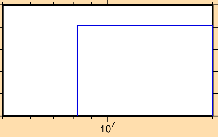
\sigma vs. E for ^{209}\text{Rn}(n,2np)
