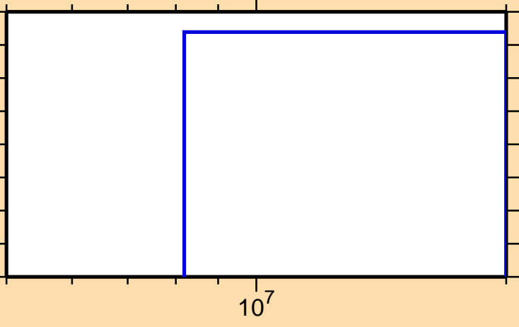
\sigma vs. E for ^{209}\text{Rn}(\text{mt117})
