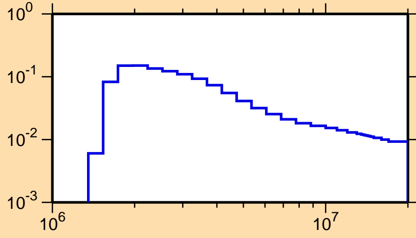
\sigma vs. E for ^{210}\text{Rn}(n,n_2)
