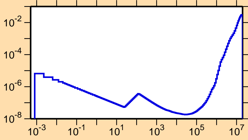
\sigma vs. E for ^{210}\text{Rn}(n,p)
