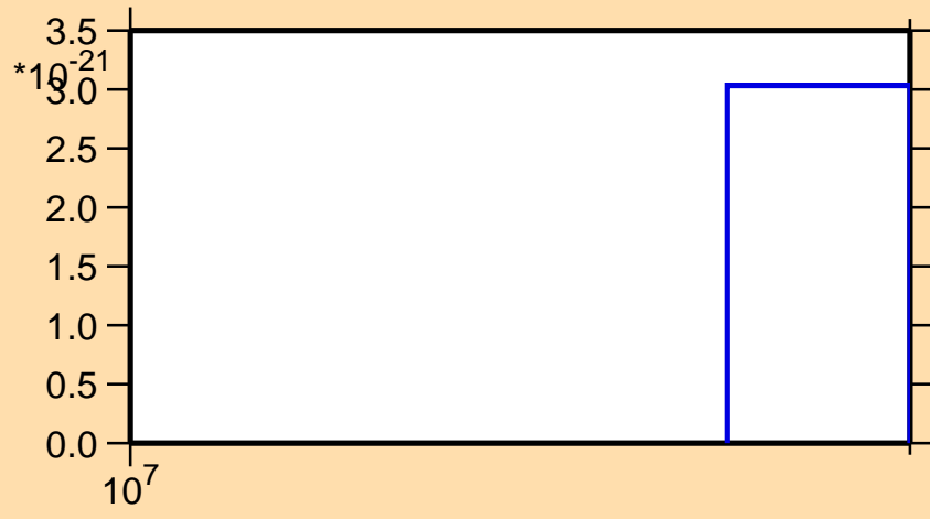
\sigma vs. E for ^{210}\text{Rn} (mt 42)
