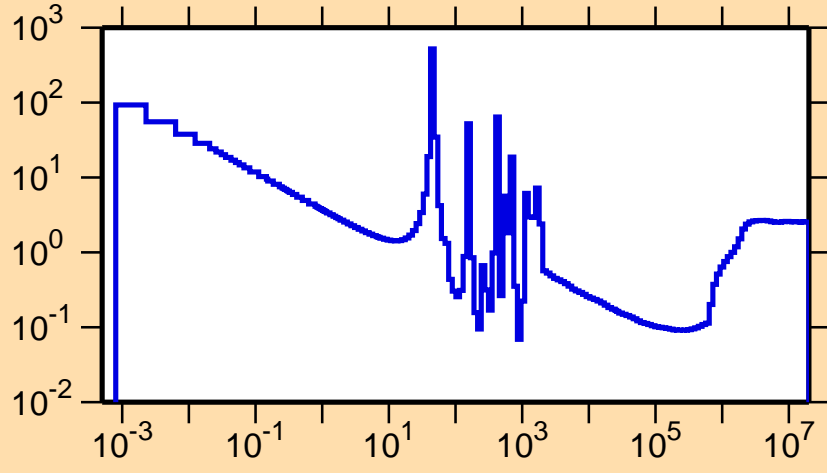
\sigma vs. E for ^{210}\text{Rn}(n,\text{nonel.})
