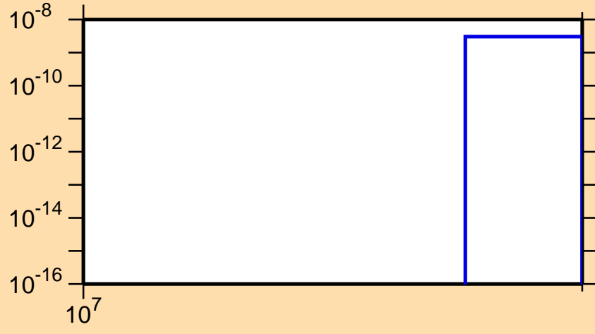
\sigma vs. E for ^{210}\text{Rn}(n,3n\alpha)
