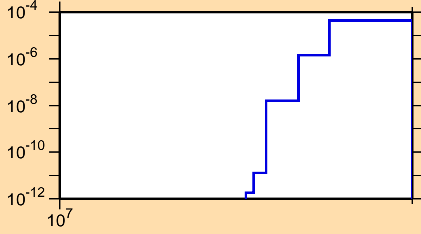
\sigma vs. E for ^{210}\text{Rn}(n,2np)
