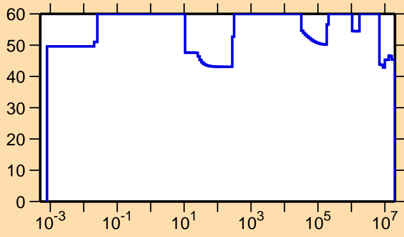
\Delta\sigma/\sigma vs. E for ^{210}\text{Rn}(n,p)
