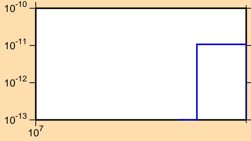
\sigma vs. E for ^{210}\text{Rn} (mt 34)
