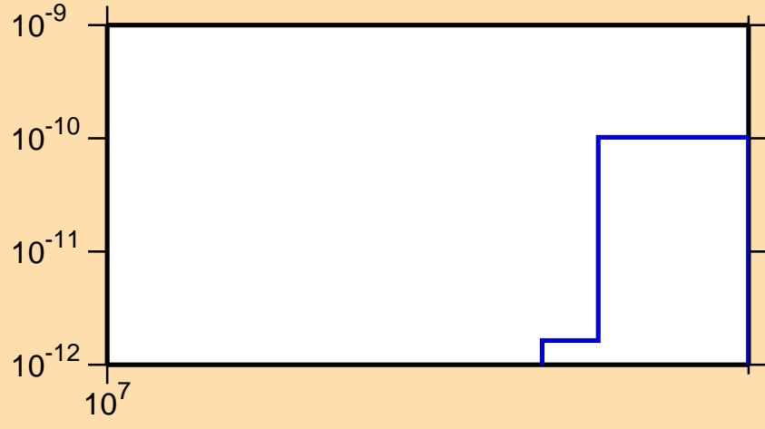
\sigma vs. E for ^{210}\text{Rn}(n,pt)
