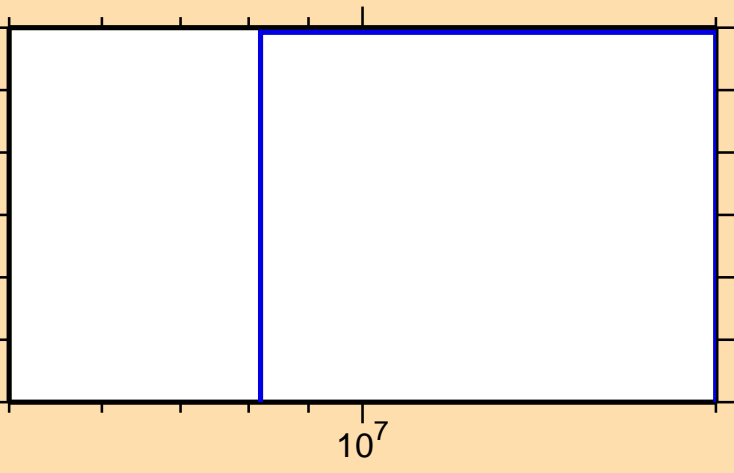
\sigma vs. E for ^{210}\text{Rn}(n,2n\alpha)
