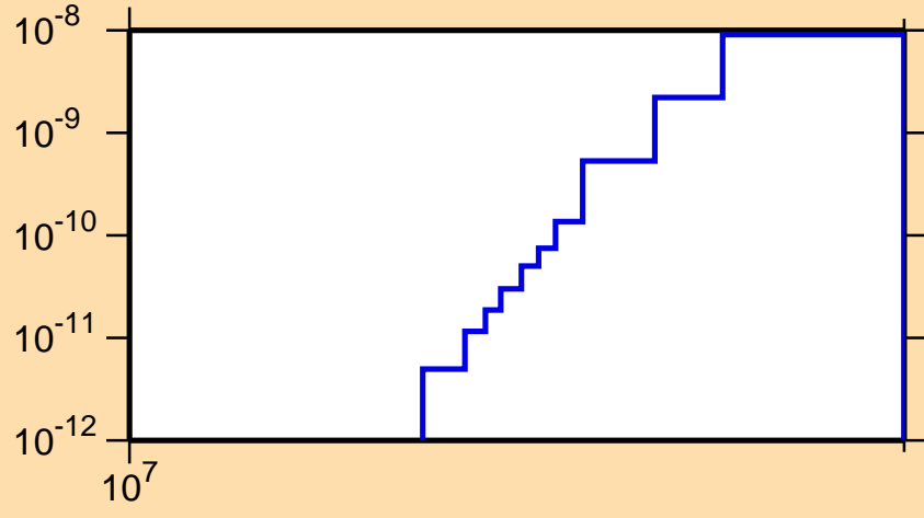
\sigma vs. E for ^{211}\text{Rn} (mt 45)
