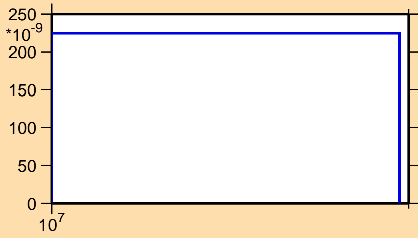
\sigma vs. E for ^{211}\text{Rn}(n,\text{nd})
