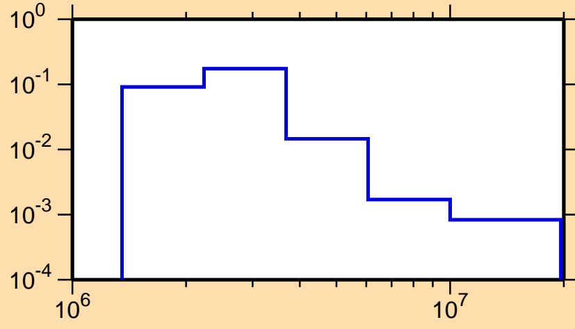
\sigma vs. E for ^{211}\text{Rn}(n,n_3)
