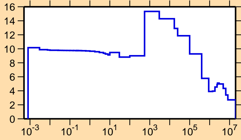
\sigma vs. E for ^{211}\text{Rn}(n,\text{el.})
