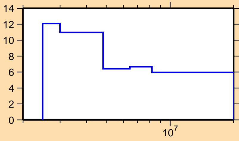
\Delta\sigma/\sigma vs. E for ^{211}\text{Rn}(n,n\text{onel.})
