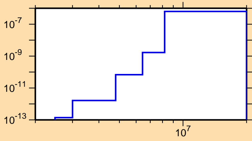
\sigma vs. E for ^{211}\text{Rn}(n,p\alpha)
