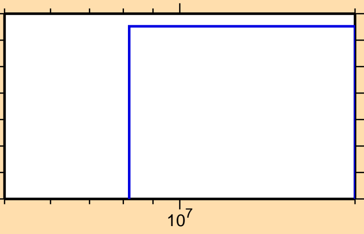
\sigma vs. E for ^{211}\text{Rn}(n,2n\alpha)
