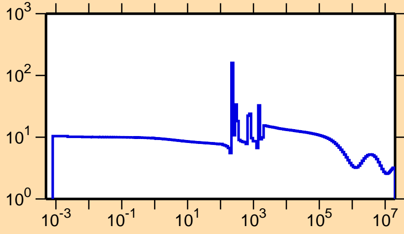
\sigma vs. E for ^{220}\text{Rn}(n,\text{el.})
