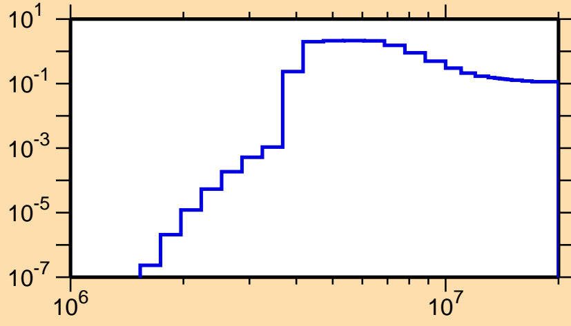
\sigma vs. E for ^{220}\text{Rn}(n,n\text{cont.})
