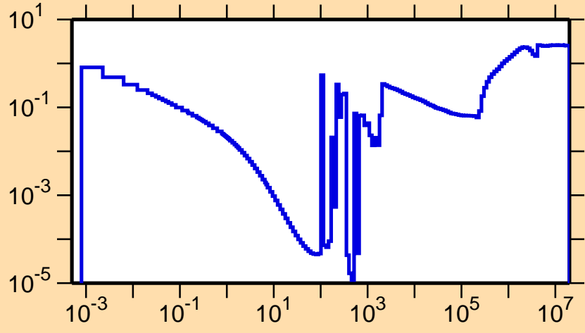
\sigma vs. E for ^{220}\text{Rn}(n,\text{nonel.})
