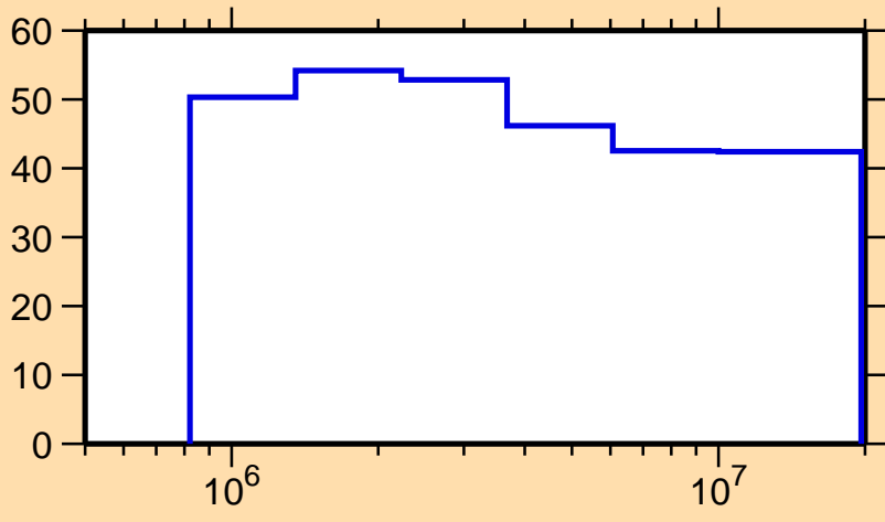
\Delta\sigma/\sigma vs. E for ^{220}\text{Rn}(n,n\text{nonel.})
