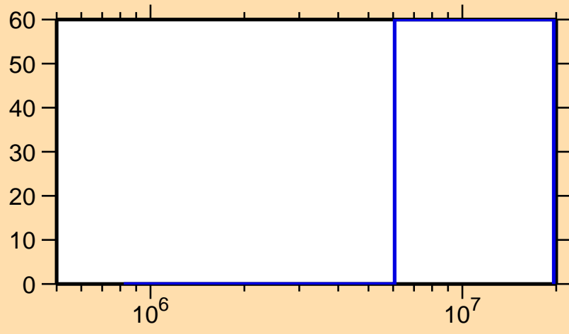
\Delta\sigma/\sigma vs. E for ^{220}\text{Rn}(n,f)
