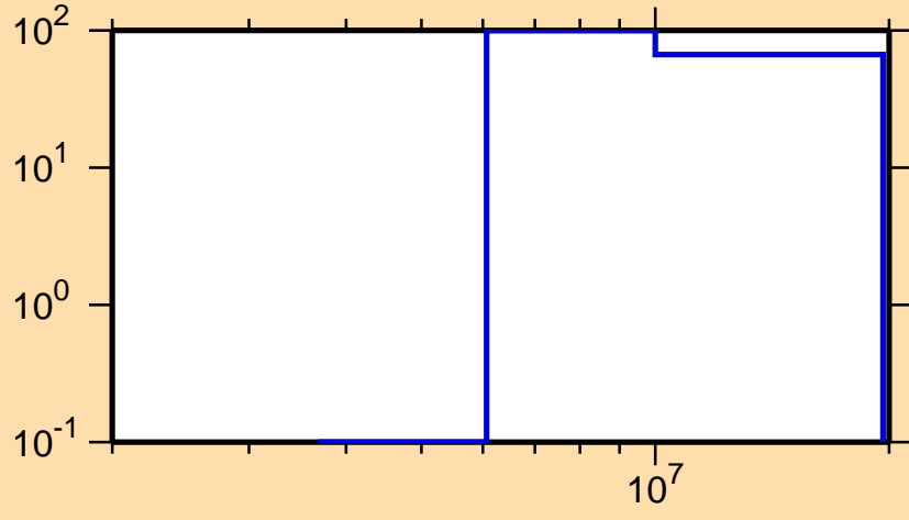
\Delta\sigma/\sigma vs. E for ^{220}\text{Rn}(n,p)
