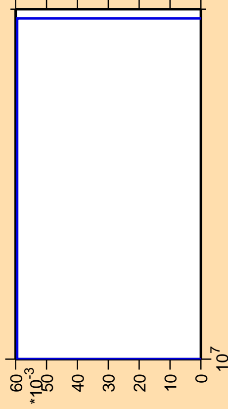
\Delta\sigma/\sigma vs. E for ^{220}\text{Rn} (mt 45)
