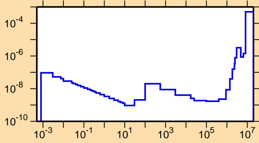
\sigma vs. E for ^{220}\text{Rn}(n,\alpha)
