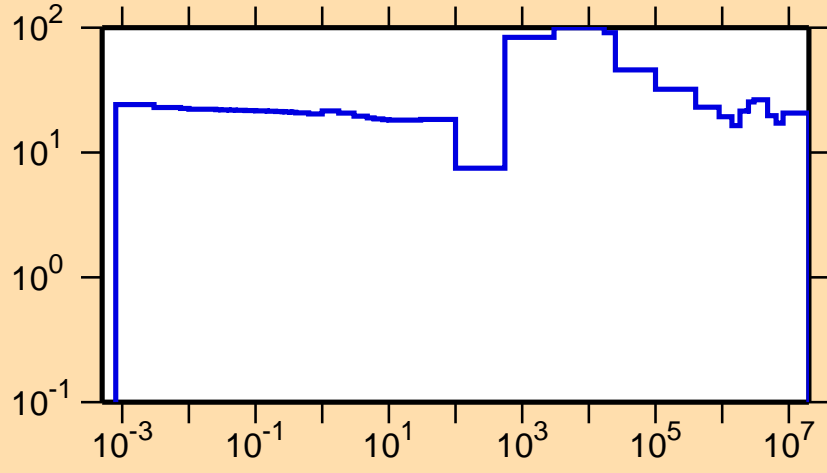
\Delta\sigma/\sigma vs. E for ^{220}\text{Rn}(n,tot.)
