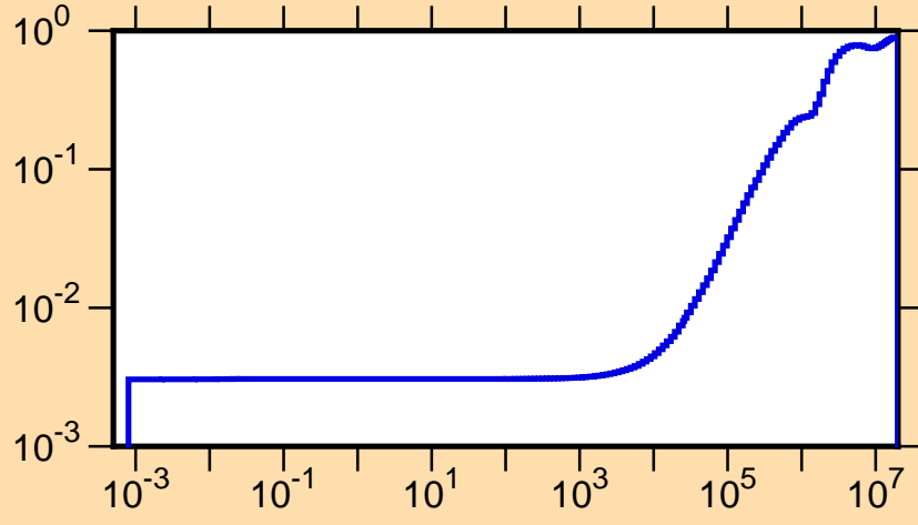
\mu vs. E for ^{221}\text{Rn}(\text{mt251})
