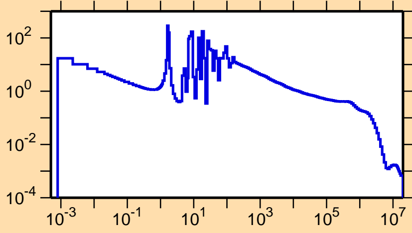
\sigma vs. E for ^{221}\text{Rn}(n,\gamma)
