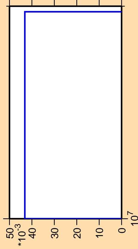
\Delta\sigma/\sigma vs. E for ^{221}\text{Rn} (mt 11)
