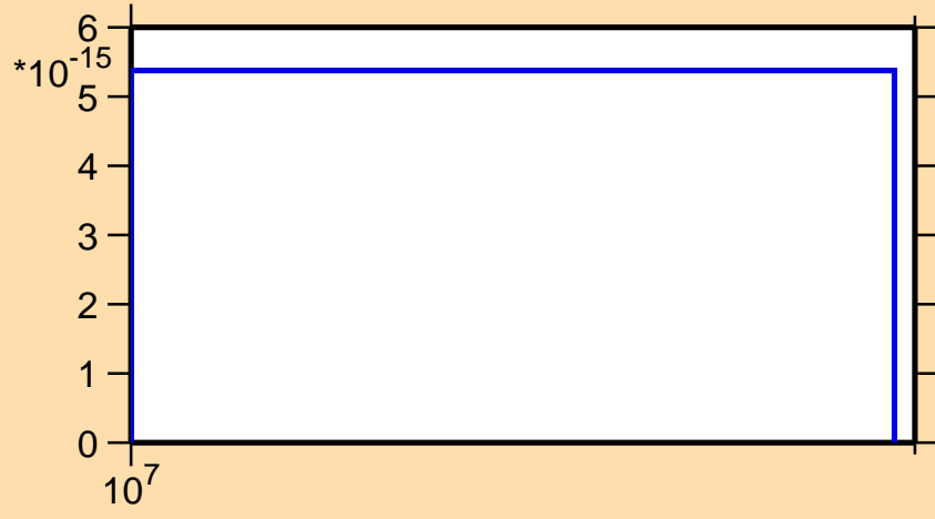
\sigma vs. E for ^{221}\text{Rn} (mt 11)
