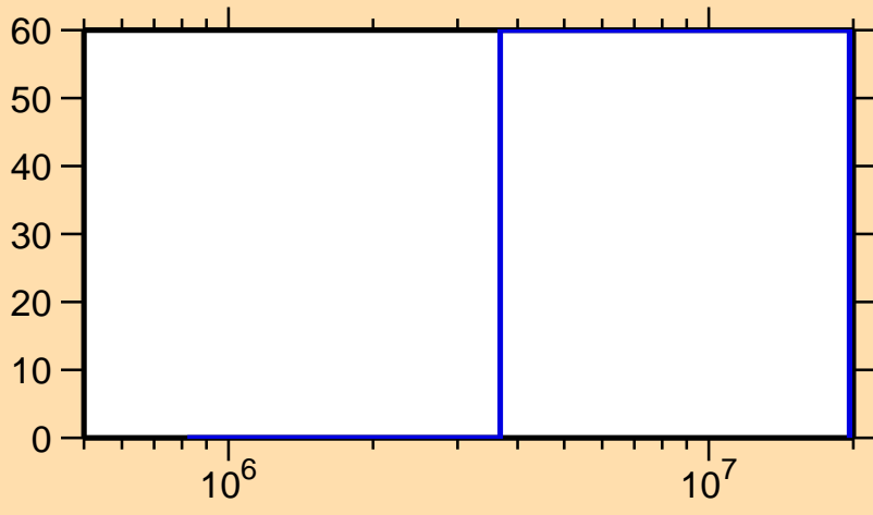
\Delta\sigma/\sigma vs. E for ^{221}\text{Rn}(n,f)
