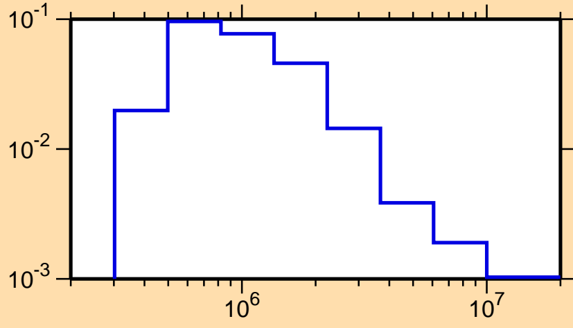
\sigma vs. E for ^{221}\text{Rn}(n,n_2)
