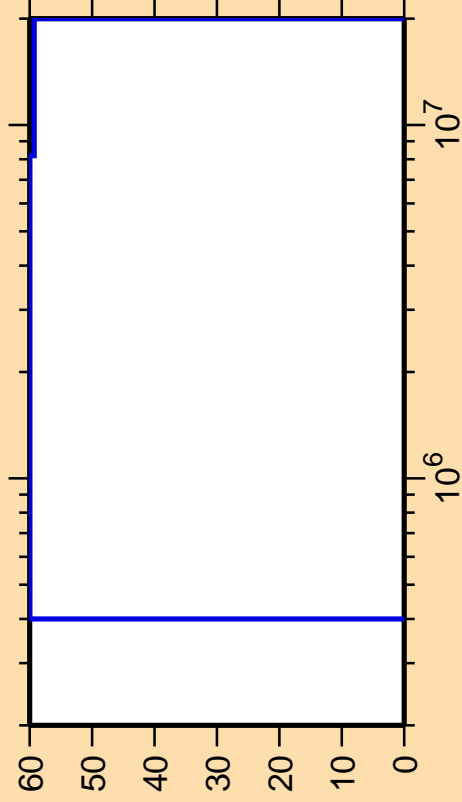
\Delta\sigma/\sigma vs. E for ^{221}\text{Rn}(n,n_3)
