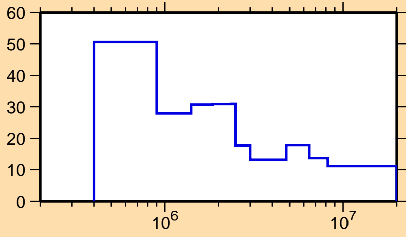
\Delta\sigma/\sigma vs. E for ^{221}\text{Rn}(n,n\text{onel.})
