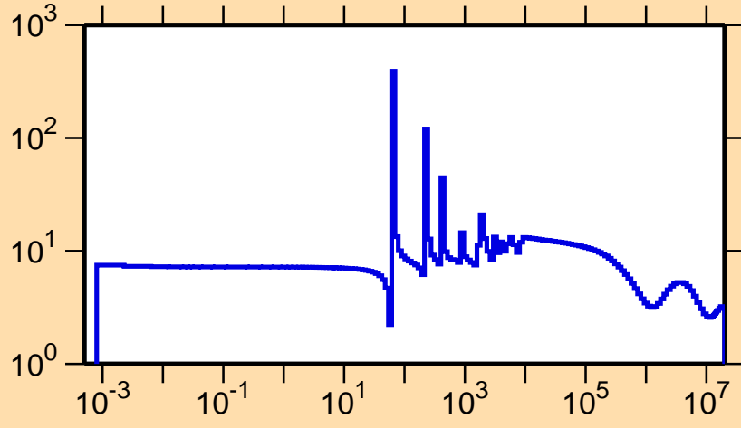
\sigma vs. E for ^{222}\text{Rn}(n,\text{el.})
