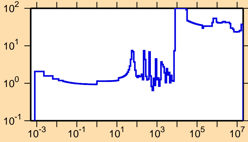
\Delta\sigma/\sigma vs. E for ^{222}\text{Rn}(n,tot.)
