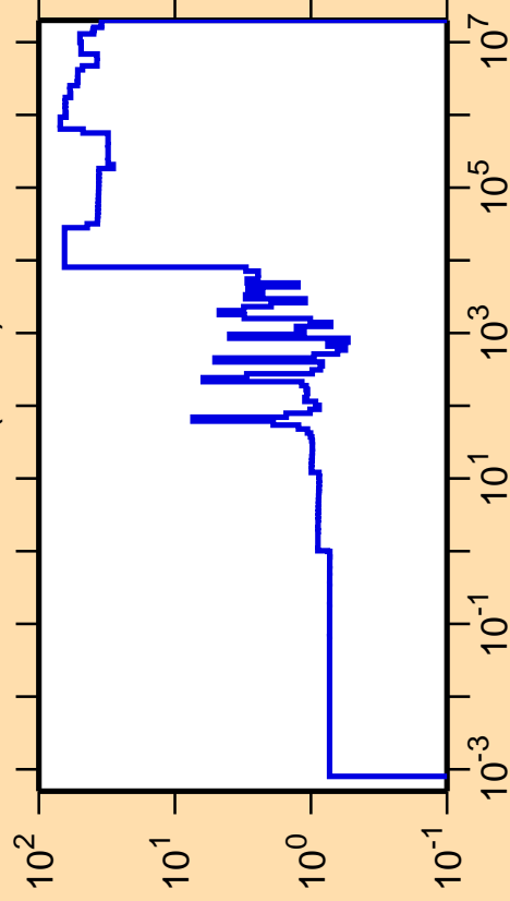
\Delta\sigma/\sigma vs. E for ^{222}\text{Rn}(n,\text{el.})
