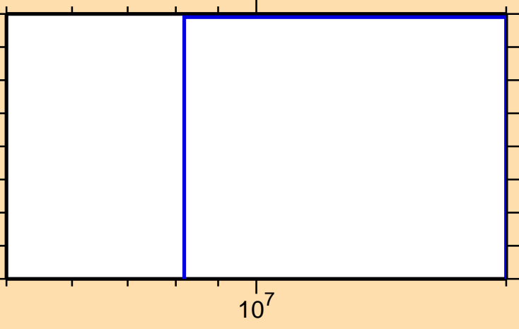
\sigma vs. E for ^{222}\text{Rn}(n,d)
