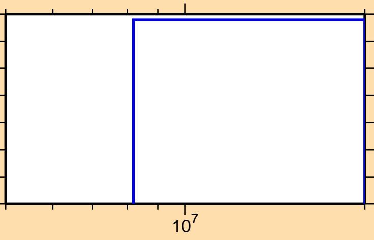
\sigma vs. E for ^{222}\text{Rn}(n,3n\alpha)
