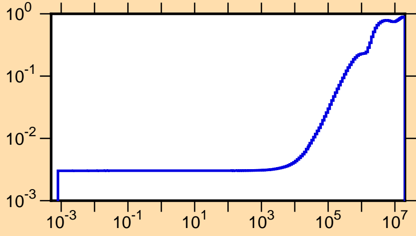
\mu vs. E for ^{223}\text{Rn}(\text{mt251})
