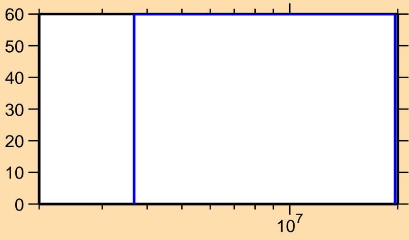
\Delta\sigma/\sigma vs. E for ^{223}\text{Rn}(n,2n)
