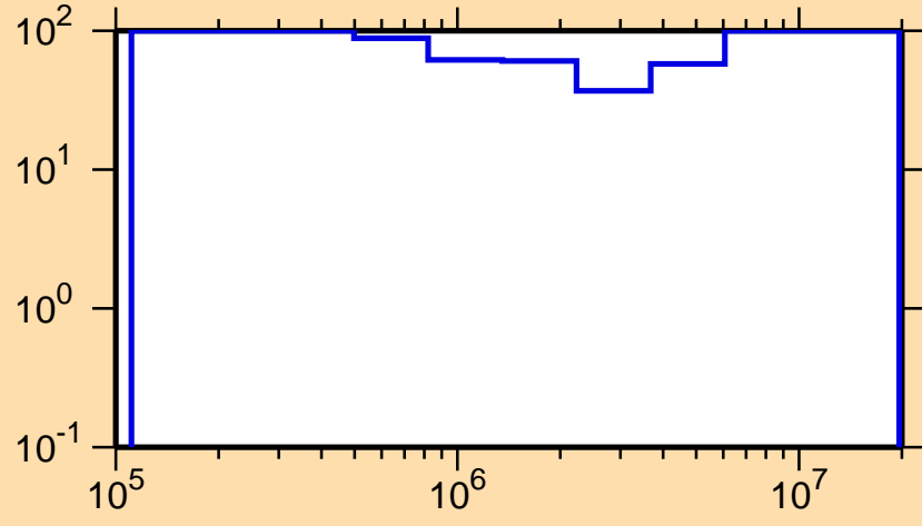
\Delta\sigma/\sigma vs. E for ^{223}\text{Rn}(n,n\text{cont.})
