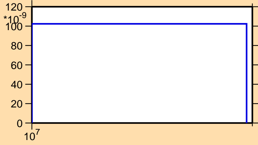
\sigma vs. E for ^{223}\text{Rn}(n,nt)
