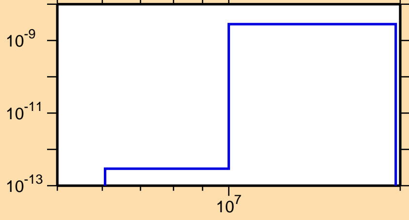
\sigma vs. E for ^{223}\text{Rn}(n,3n\alpha)
