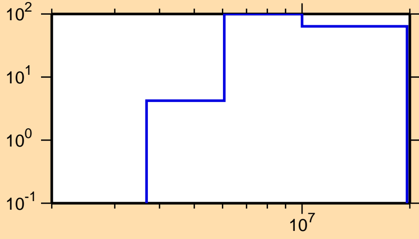
\Delta\sigma/\sigma vs. E for ^{223}\text{Rn}(n,p)
