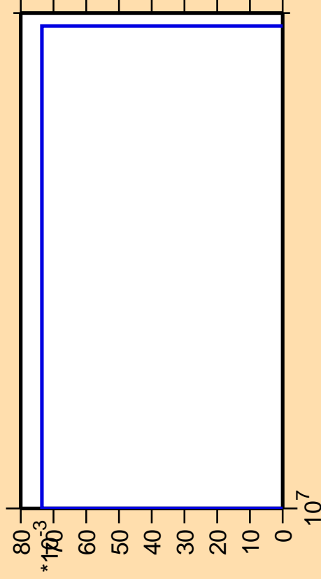
\Delta\sigma/\sigma vs. E for ^{223}\text{Rn}(n,\text{He3})
