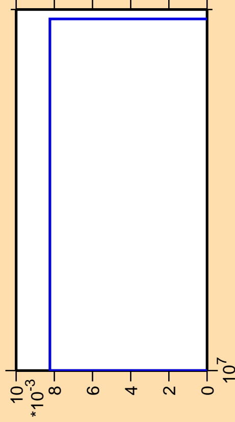
\Delta\sigma/\sigma vs. E for ^{223}\text{Rn} (mt 11)
