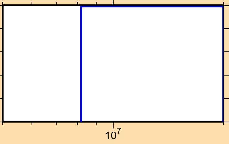
\sigma vs. E for ^{223}\text{Rn}(n,t)
