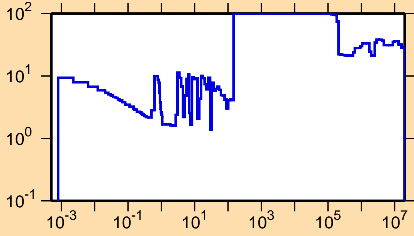
\Delta\sigma/\sigma vs. E for ^{225}\text{Rn}(n,\text{tot.})
