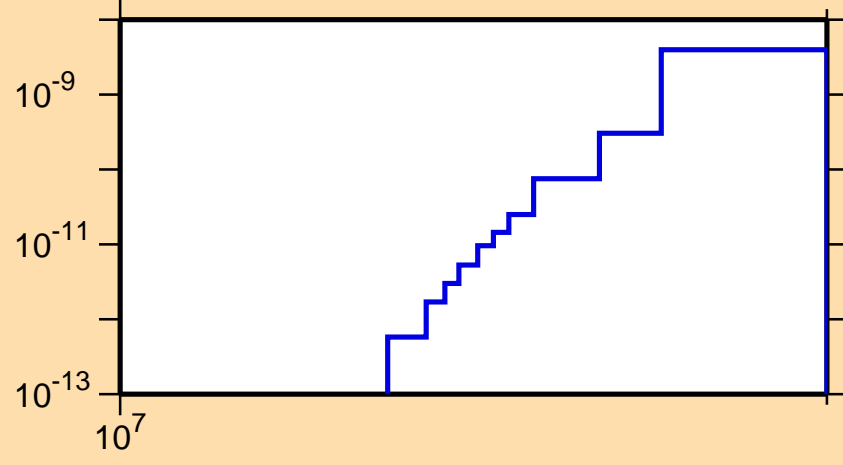
\sigma vs. E for ^{225}\text{Rn}(n,3n\alpha)
