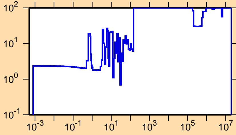
\Delta\sigma/\sigma vs. E for ^{225}\text{Rn}(n,\text{el.})
