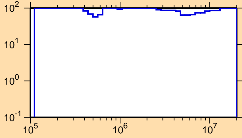
\Delta\sigma/\sigma vs. E for ^{225}\text{Rn}(n,\text{inel.})
