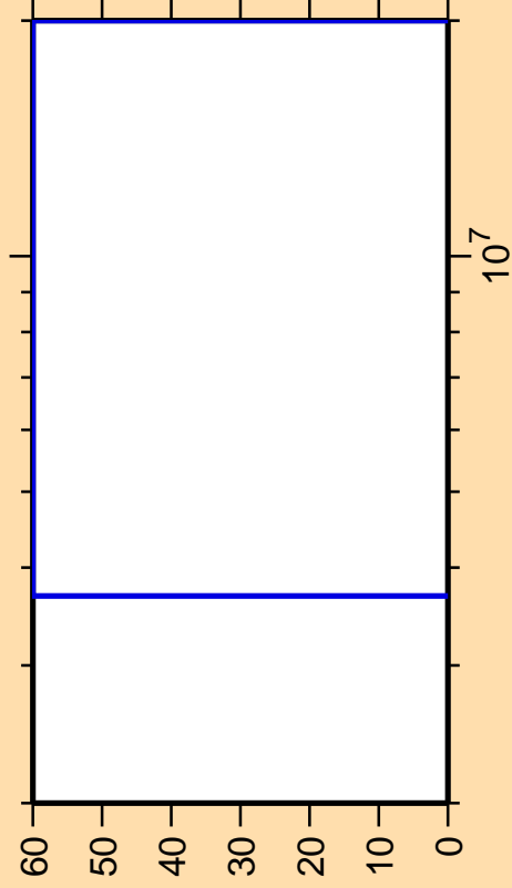
\Delta\sigma/\sigma vs. E for ^{225}\text{Rn}(n,n\text{cont.})
