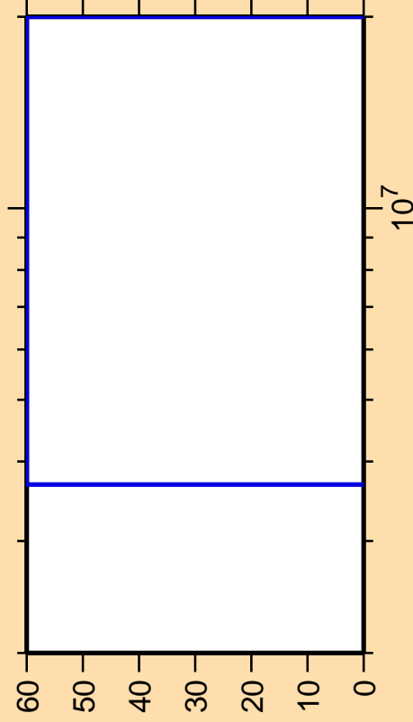
\Delta\sigma/\sigma vs. E for ^{225}\text{Rn}(n,2n)
