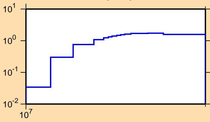
\sigma vs. E for ^{225}\text{Rn}(n,3n)
