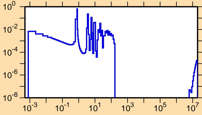
\sigma vs. E for ^{225}\text{Rn}(n,f)
