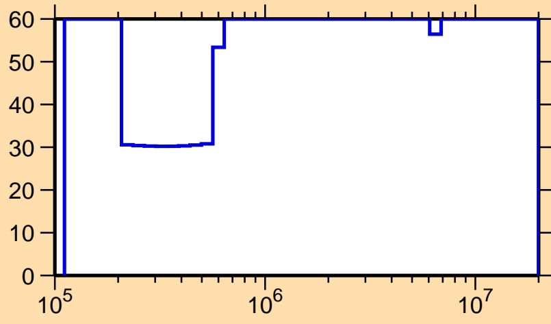
\Delta\sigma/\sigma vs. E for ^{225}\text{Rn}(n,\text{el.})
