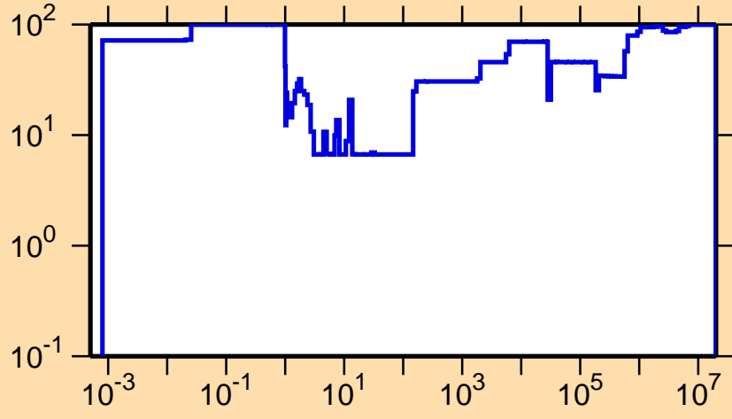
\Delta\sigma/\sigma vs. E for ^{225}\text{Rn}(n,\text{nonel.})
