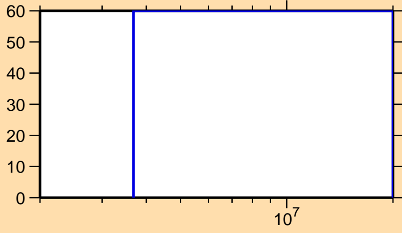
\Delta\sigma/\sigma vs. E for ^{225}\text{Rn}(n,2n)
