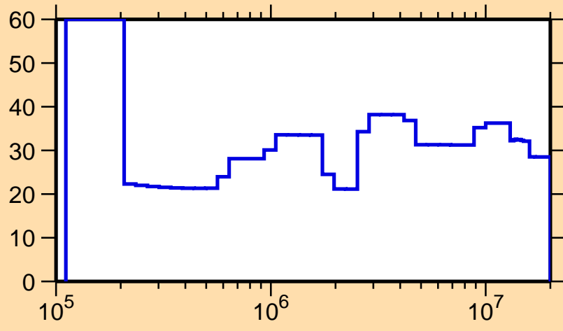
\Delta\sigma/\sigma vs. E for ^{225}\text{Rn}(n,\text{tot.})
