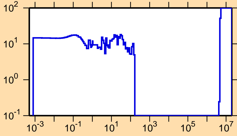
\Delta\sigma/\sigma vs. E for ^{225}\text{Rn}(n,f)
