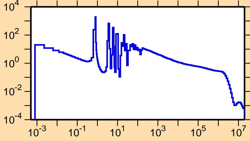
\sigma vs. E for ^{225}\text{Rn}(n,\gamma)
