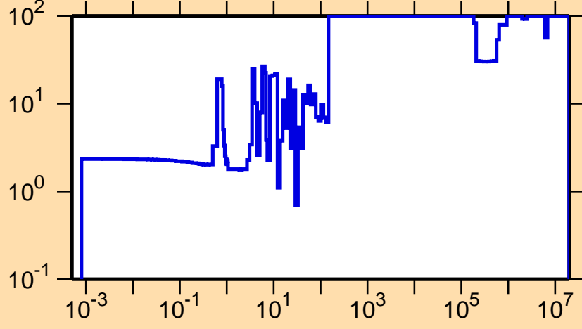
\Delta\sigma/\sigma vs. E for ^{225}\text{Rn}(n,el.)
