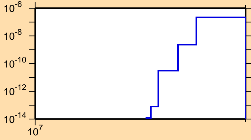
\sigma vs. E for ^{225}\text{Rn}(n,2np)
