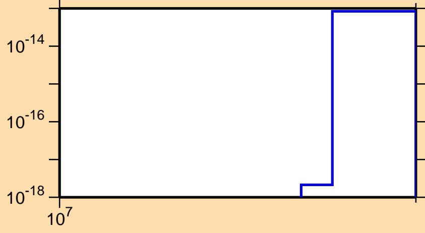
\sigma vs. E for ^{225}\text{Rn}(n,\text{He}3)
