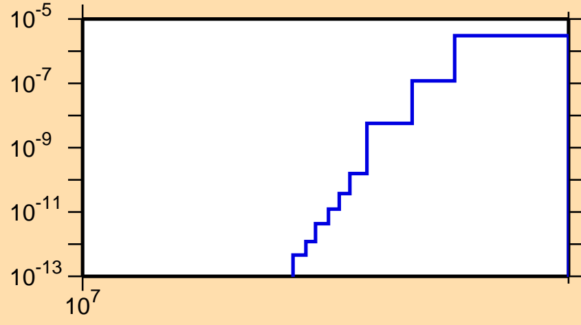
\sigma vs. E for ^{225}\text{Rn}(n,nt)
