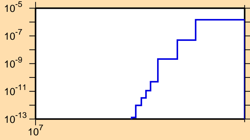
\sigma vs. E for ^{225}\text{Rn}(n,nd)
