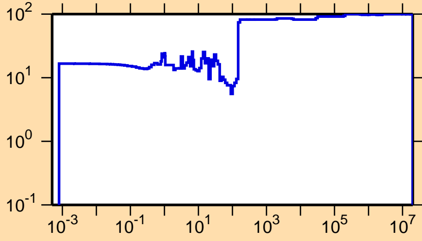
\Delta\sigma/\sigma vs. E for ^{225}\text{Rn}(n,\gamma)
