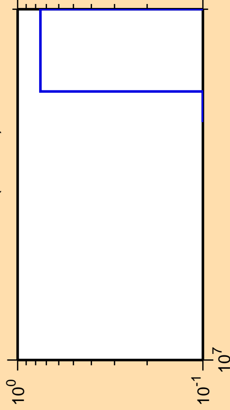
\Delta\sigma/\sigma vs. E for ^{225}\text{Rn}(n,\text{He}3)
