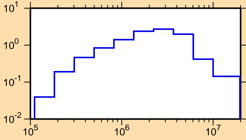
\sigma vs. E for ^{225}\text{Rn}(n,\text{inel.})
