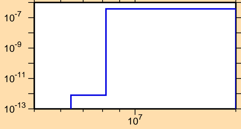
\sigma vs. E for ^{225}\text{Rn}(n,2n\alpha)
