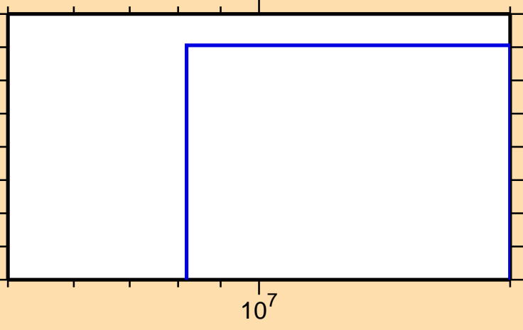
\sigma vs. E for ^{225}\text{Rn}(n,\text{nd})
