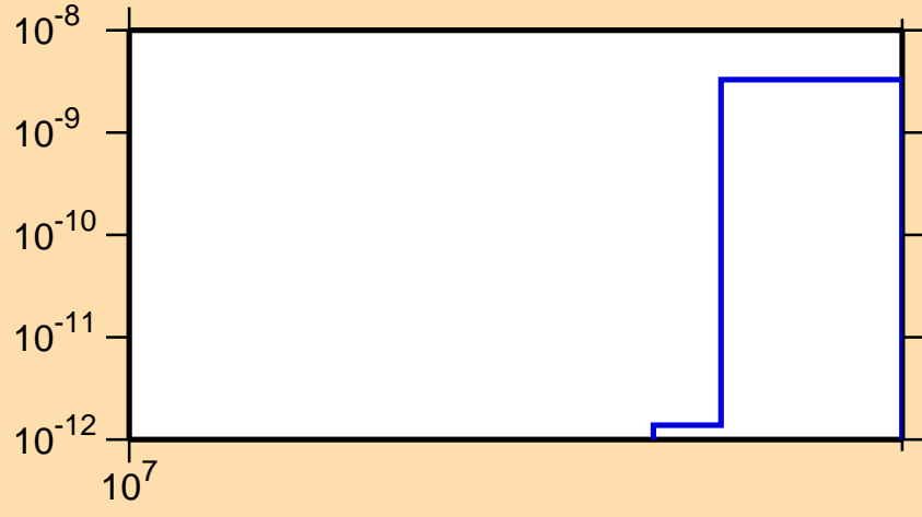
\sigma vs. E for ^{228}\text{Rn}(n,\text{nd})
