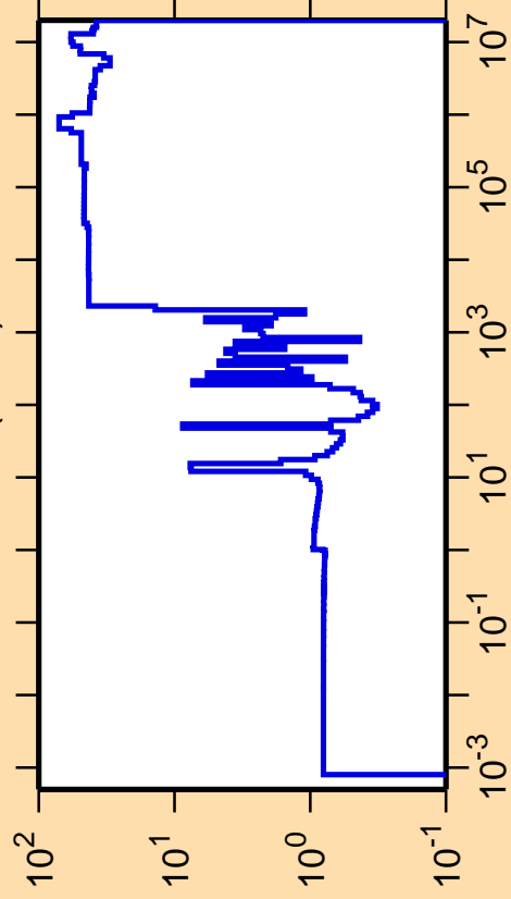
\Delta\sigma/\sigma vs. E for ^{228}\text{Rn}(n,\text{el.})
