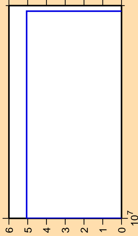
\Delta\sigma/\sigma vs. E for ^{228}\text{Rn}(n,2np)
