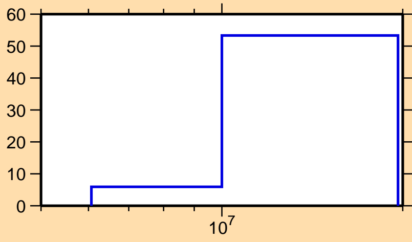
\Delta\sigma/\sigma vs. E for ^{228}\text{Rn}(n,p)
