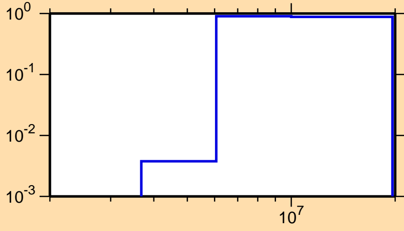
\sigma vs. E for ^{228}\text{Rn}(n,2n)
