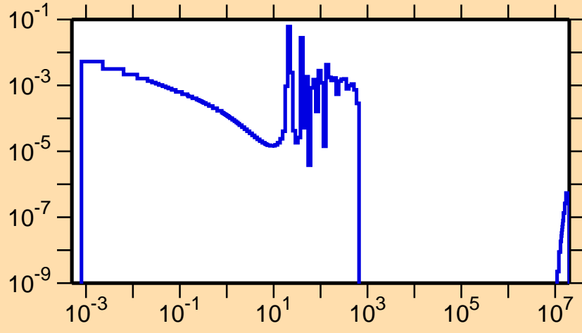
\sigma vs. E for ^{229}\text{Rn}(n,f)
