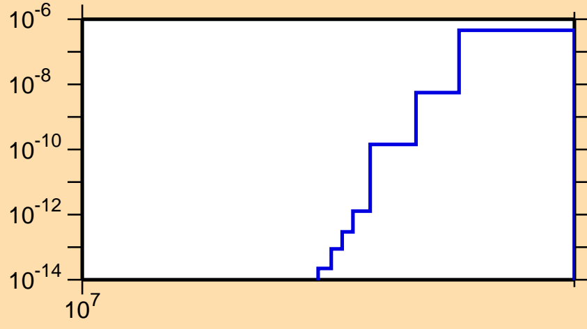
\sigma vs. E for ^{229}\text{Rn}(n,nt)
