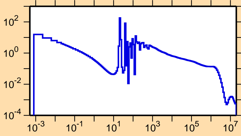
\sigma vs. E for ^{229}\text{Rn}(n,\gamma)
