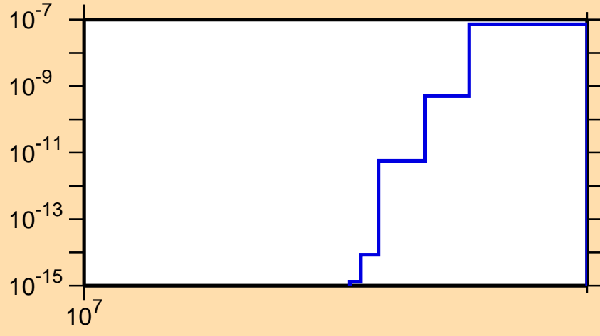
\sigma vs. E for ^{229}\text{Rn}(n,nd)
