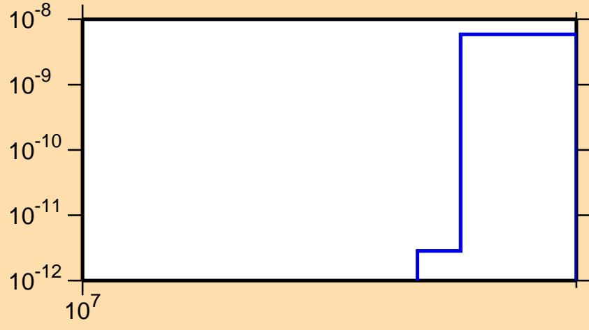
\sigma vs. E for ^{229}\text{Rn}(n,2np)
