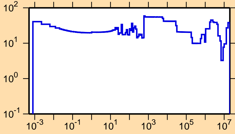
\Delta\sigma/\sigma vs. E for ^{229}\text{Rn}(n,tot.)
