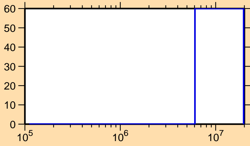
\Delta\sigma/\sigma vs. E for ^{229}\text{Rn}(n,f)
