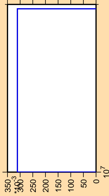
\Delta\sigma/\sigma vs. E for ^{229}\text{Rn}(n,3n\alpha)
