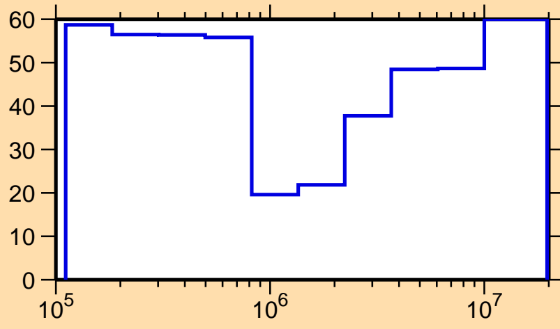
\Delta\sigma/\sigma vs. E for ^{229}\text{Rn}(n,\text{inel.})
