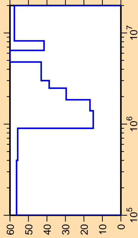
\Delta\sigma/\sigma vs. E for ^{229}\text{Rn}(n,\text{inel.})
