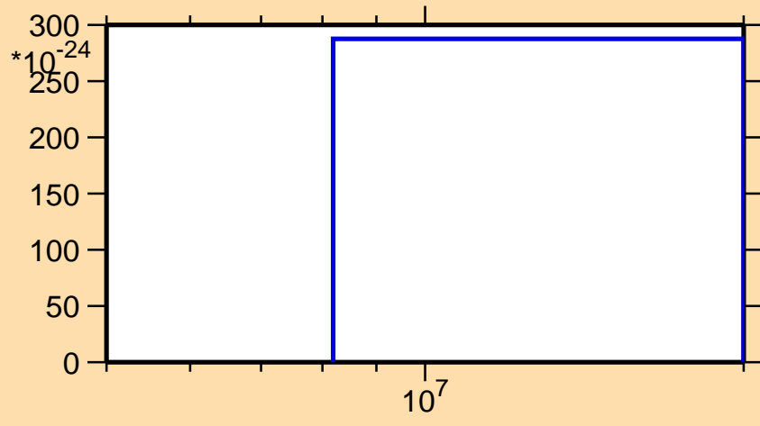
\sigma vs. E for ^{229}\text{Rn} (mt 42)
