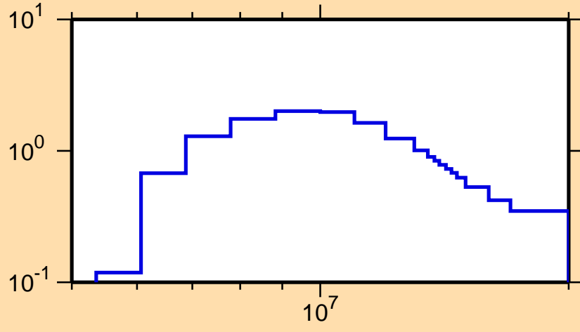
\sigma vs. E for ^{230}\text{Rn}(n,2n)
