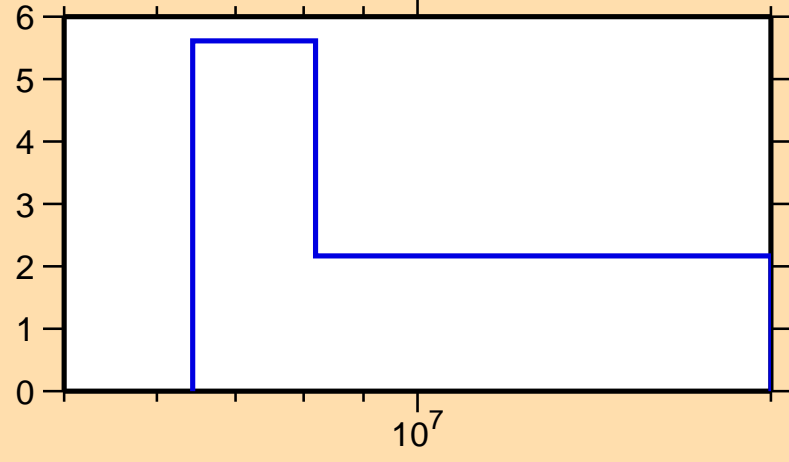
\Delta\sigma/\sigma vs. E for ^{230}\text{Rn}(n,\text{tot.})
