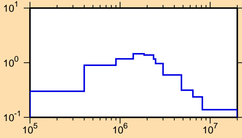
\sigma vs. E for ^{230}\text{Rn}(n,n_1)
