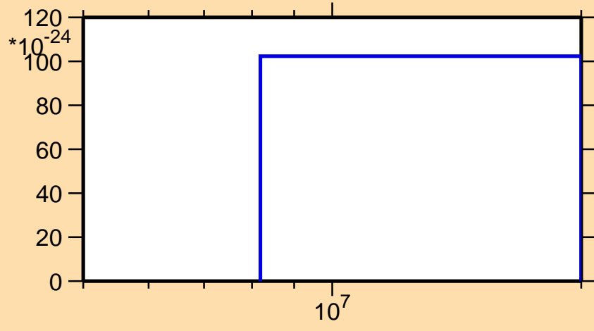
\sigma vs. E for ^{230}\text{Rn} (mt 42)
