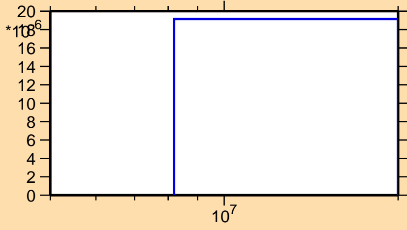
\sigma vs. E for ^{230}\text{Rn}(n,p)
