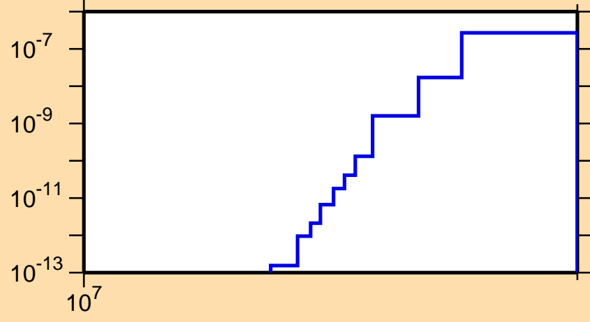
\sigma vs. E for ^{88}\text{Ru} (mt 45)
