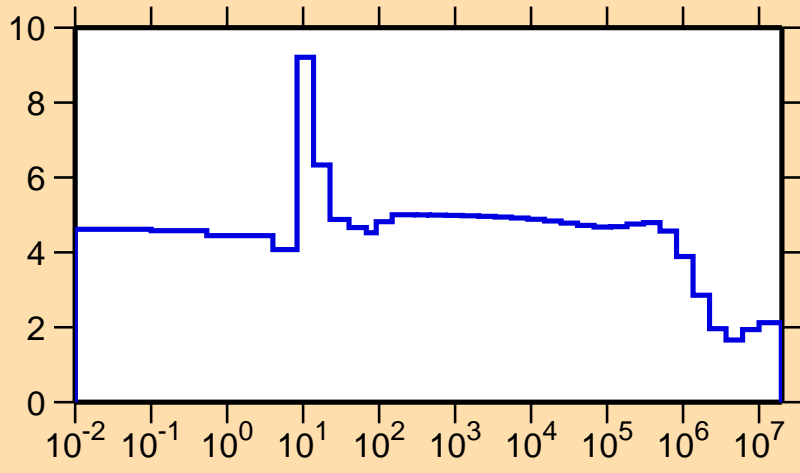
\sigma vs. E for ^{88}\text{Ru}(n,\text{el.})
