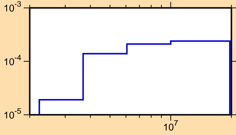
\sigma vs. E for ^{88}\text{Ru}(n,n_3)
