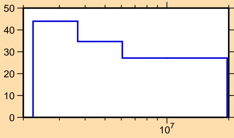
\Delta\sigma/\sigma vs. E for ^{88}\text{Ru}(n,ncont.)
