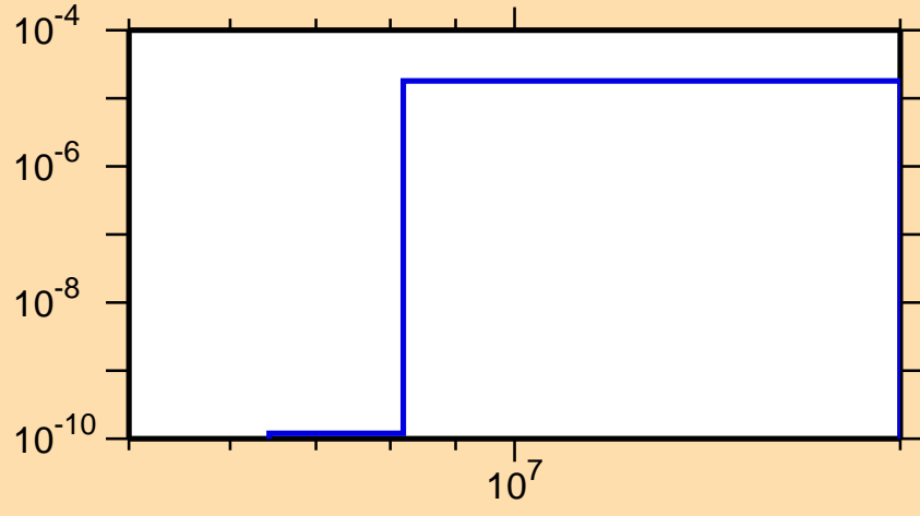
\sigma vs. E for ^{88}\text{Ru}(n,n\alpha)
