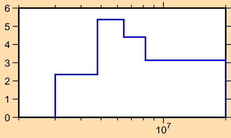
\Delta\sigma/\sigma vs. E for ^{88}\text{Ru}(n,n\text{nonel.})
