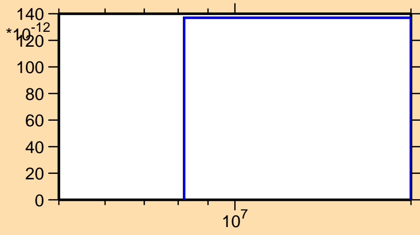
\sigma vs. E for ^{91}\text{Ru} (mt 34)
