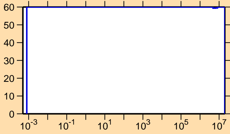
\Delta\sigma/\sigma vs. E for ^{91}\text{Ru}(n,\gamma)
