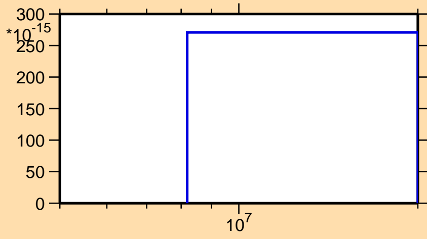
\sigma vs. E for ^{91}\text{Ru}(\text{mt117})
