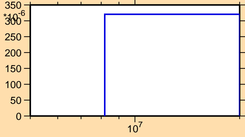
\sigma vs. E for ^{91}\text{Ru}(n,2n)
