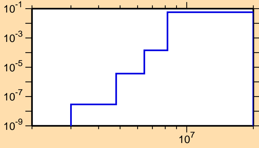
\sigma vs. E for ^{91}\text{Ru}(n,p\alpha)
