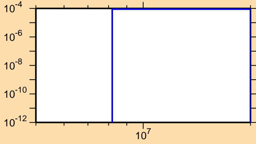
\sigma vs. E for ^{91}\text{Ru}(n,n\alpha)
