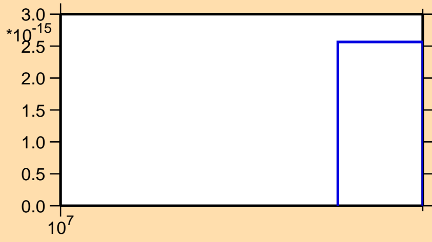
\sigma vs. E for ^{92}\text{Ru}(n,2np)
