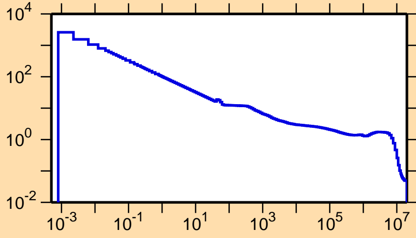
\sigma vs. E for ^{92}\text{Ru}(n,p)
