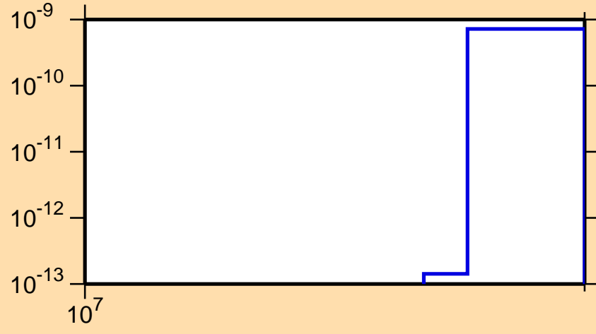
\sigma vs. E for ^{92}\text{Ru} (mt 45)
