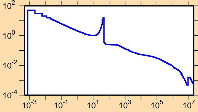
\sigma vs. E for ^{92}\text{Ru}(n,\gamma)
