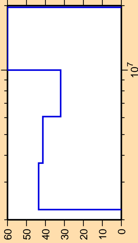
\Delta\sigma/\sigma vs. E for ^{92}\text{Ru}(n,n\text{cont.})
