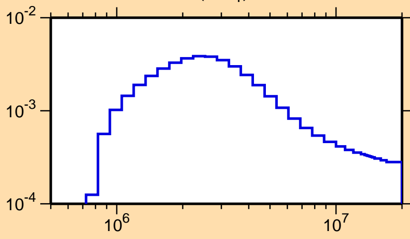
\sigma vs. E for ^{93}\text{Ru}(n,n_1)
