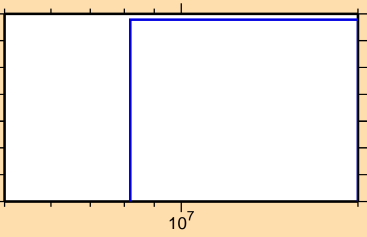
\sigma vs. E for ^{93}\text{Ru}(n,t)
