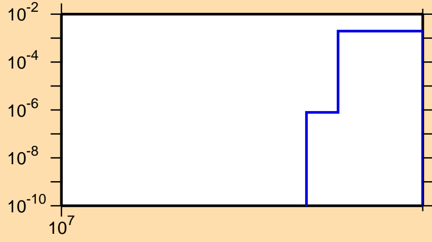
\sigma vs. E for ^{95}\text{Ru}(n,2np)
