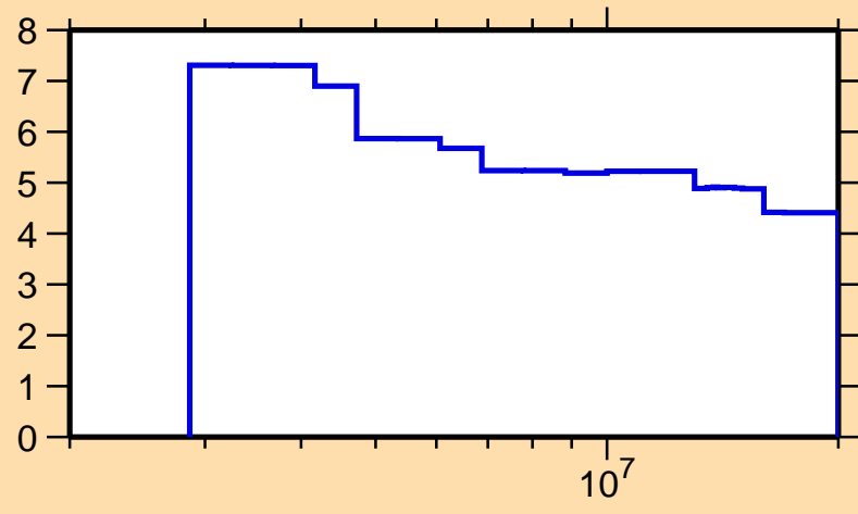
\Delta\sigma/\sigma vs. E for ^{95}\text{Ru}(n,n\text{onel.})
