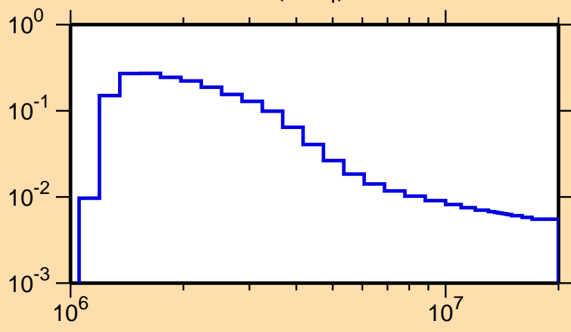
\sigma vs. E for ^{95}\text{Ru}(n,n_4)
