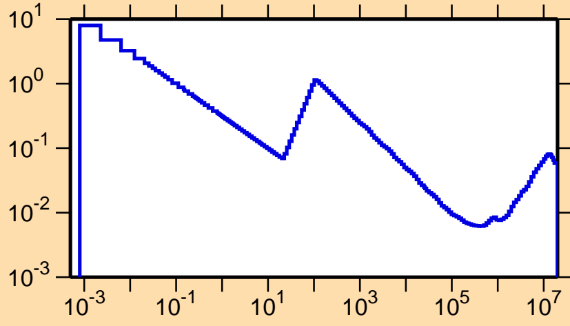
\sigma vs. E for ^{95}\text{Ru}(n,\alpha)
