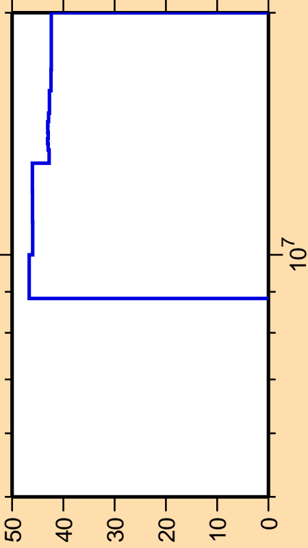
\Delta\sigma/\sigma vs. E for ^{95}\text{Ru}(n,n_1)
