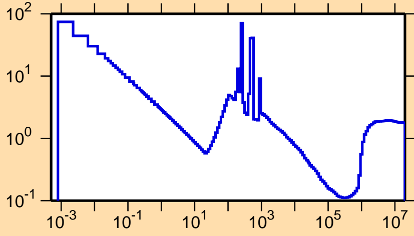
\sigma vs. E for ^{95}\text{Ru}(n,\text{nonel.})
