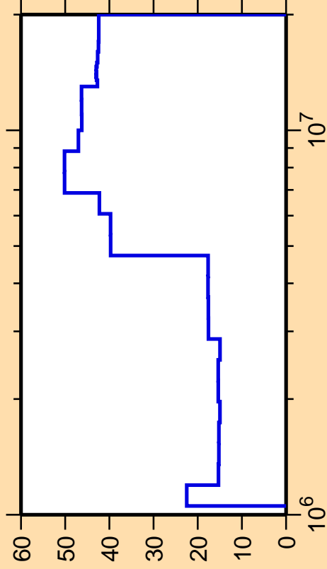
\Delta\sigma/\sigma vs. E for ^{95}\text{Ru}(n,n_4)
