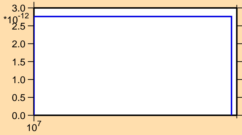
\sigma vs. E for ^{95}\text{Ru}(\text{mt } 45)
