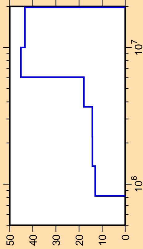
\Delta\sigma/\sigma vs. E for ^{95}\text{Ru}(n,n_2)
