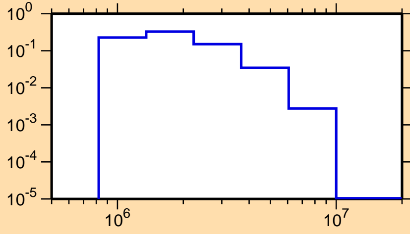
\sigma vs. E for ^{95}\text{Ru}(n,n_3)
