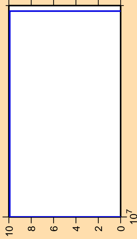
\Delta\sigma/\sigma vs. E for ^{95}\text{Ru}(\text{mt } 45)
