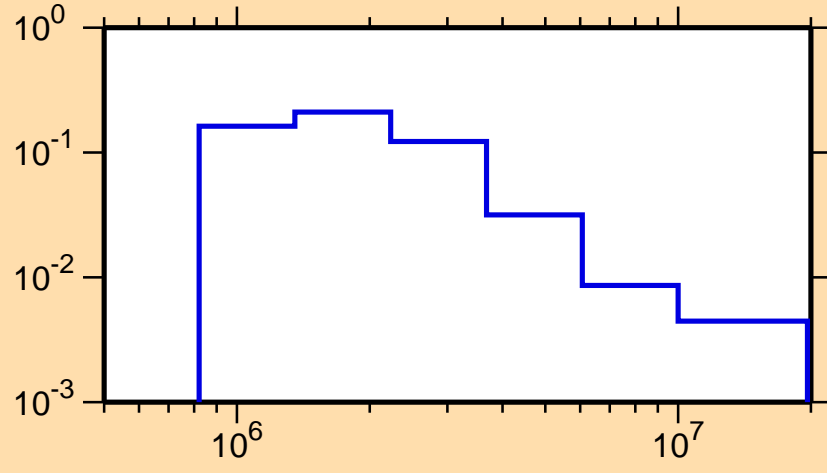
\sigma vs. E for ^{95}\text{Ru}(n,n_2)
