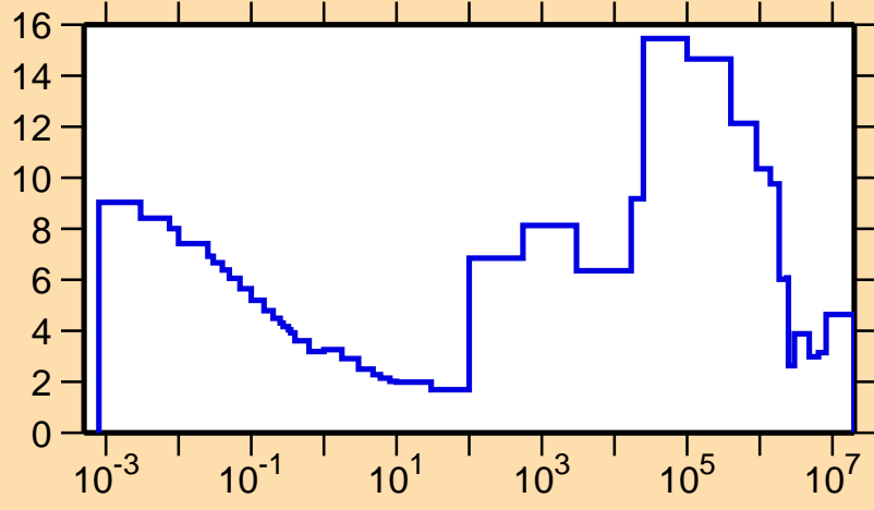
\Delta\sigma/\sigma vs. E for ^{95}\text{Ru}(n,\text{tot.})
