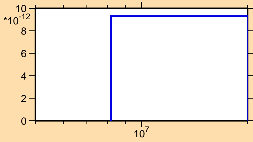
\sigma vs. E for ^{95}\text{Ru} (mt 34)
