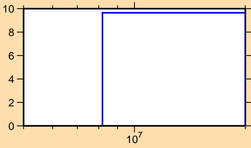
\Delta\sigma/\sigma vs. E for ^{95}\text{Ru}(n,\text{el.})
