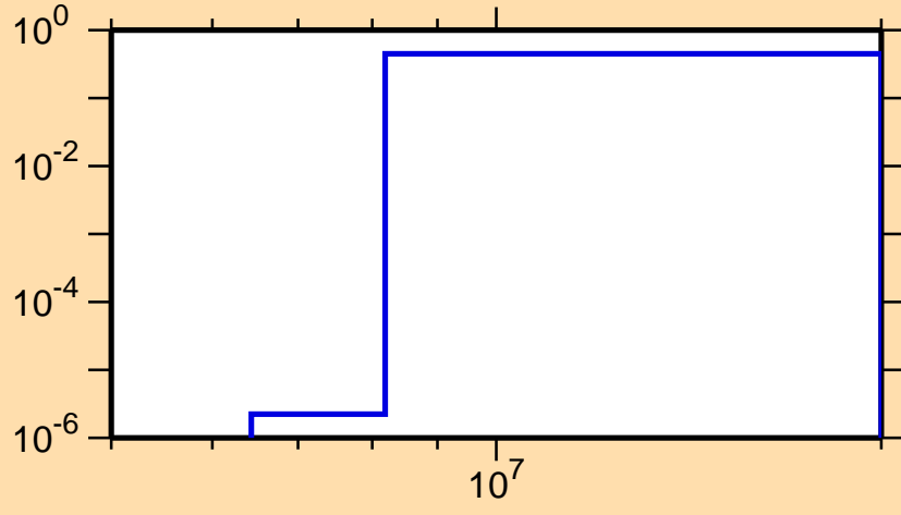
\sigma vs. E for ^{95}\text{Ru}(n,np)
