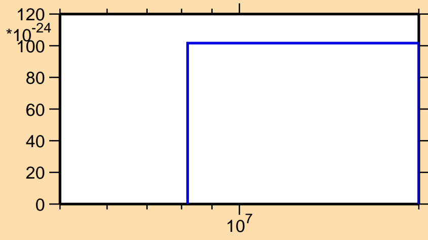
\sigma vs. E for ^{95}\text{Ru}(n,nt)
