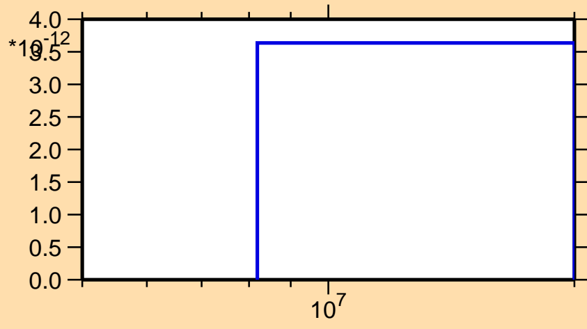
\sigma vs. E for ^{95}\text{Ru} (mt 45)
