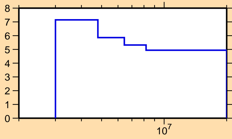
\Delta\sigma/\sigma vs. E for ^{95}\text{Ru}(n,n\text{nonel.})
