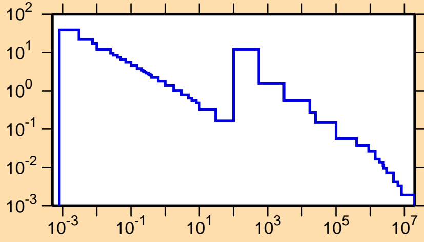
\sigma vs. E for ^{95}\text{Ru}(n,\gamma)
