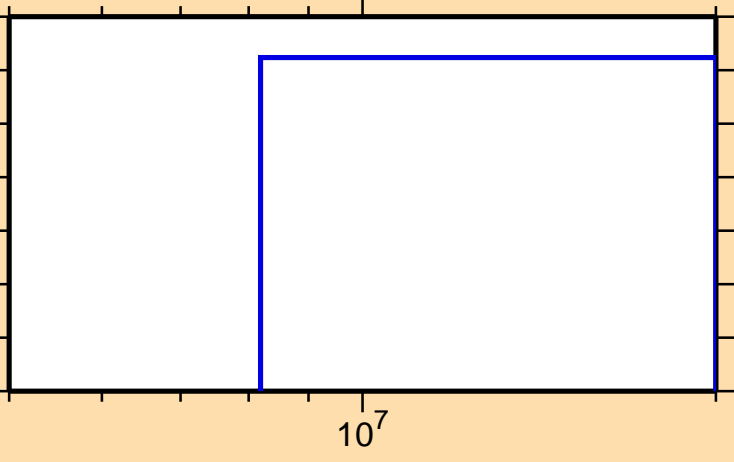
\sigma vs. E for ^{95}\text{Ru}(n,\text{pt})
