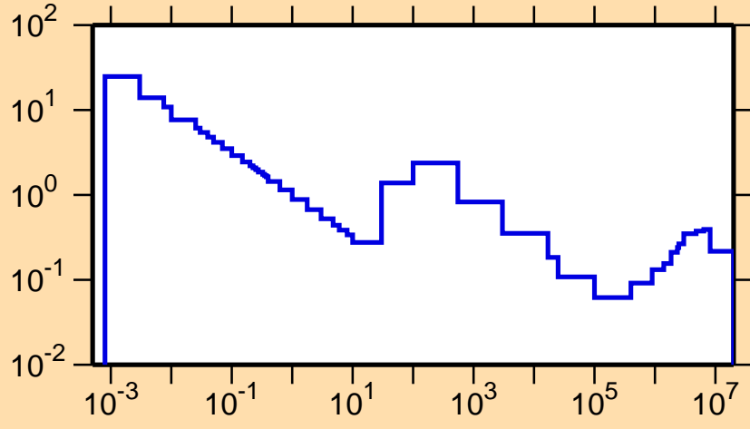
\sigma vs. E for ^{95}\text{Ru}(n,p)
