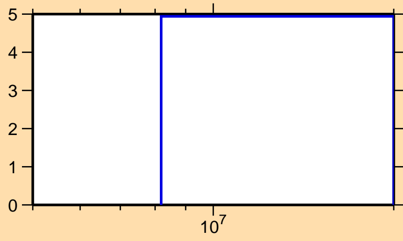
\Delta\sigma/\sigma vs. E for ^{95}\text{Ru}(n,\text{nonel.})
