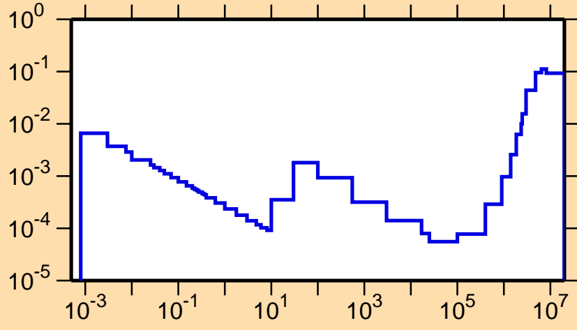
\sigma vs. E for ^{97}\text{Ru}(n,p)
