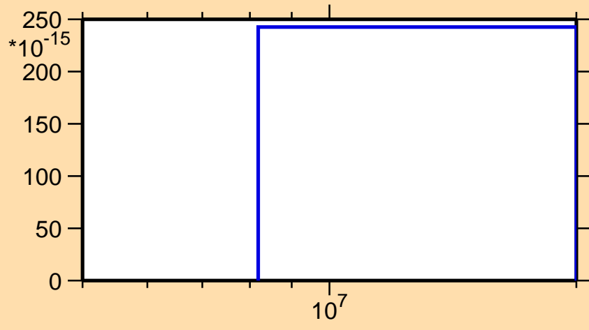
\sigma vs. E for ^{97}\text{Ru}(\text{mt } 34)
