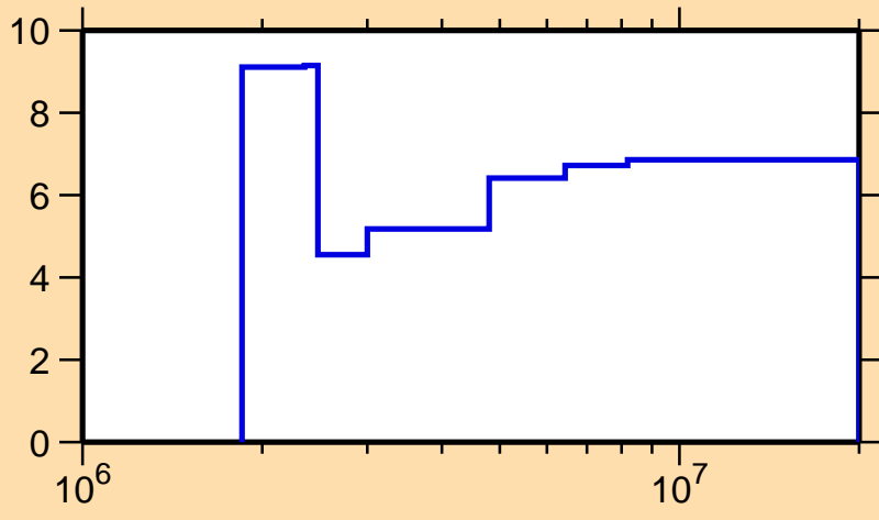
\Delta\sigma/\sigma vs. E for ^{97}\text{Ru}(n,n\text{onel.})
