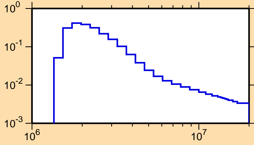
\sigma vs. E for ^{98}\text{Ru}(n,n_4)
