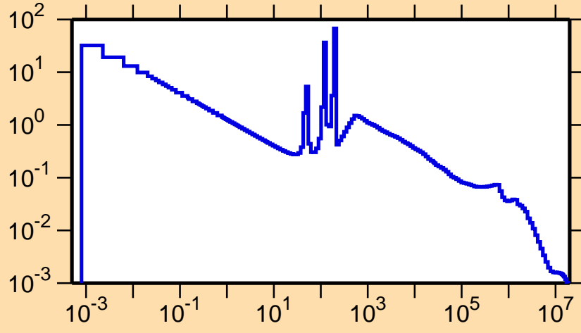
\sigma vs. E for ^{98}\text{Ru}(n,\gamma)
