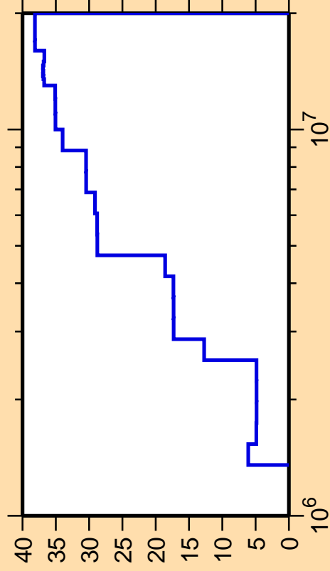
\Delta\sigma/\sigma vs. E for ^{98}\text{Ru}(n,n_4)
